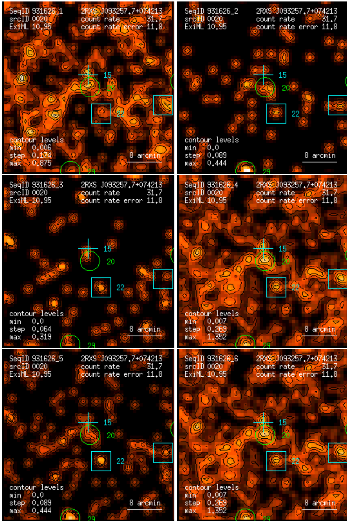
Figure 20: RASS 931626: detection 0020: band rate images, Gaussian filter: (1) PSPC channels 11 – 41, (2) 52 – 90, (3) 91 – 201, (4) 11 – 235, (5) 52 – 201, (6) 11 – 201. Broad band rates in counts/ks. Band rate contour levels in counts/ks/arcmin 2 .
