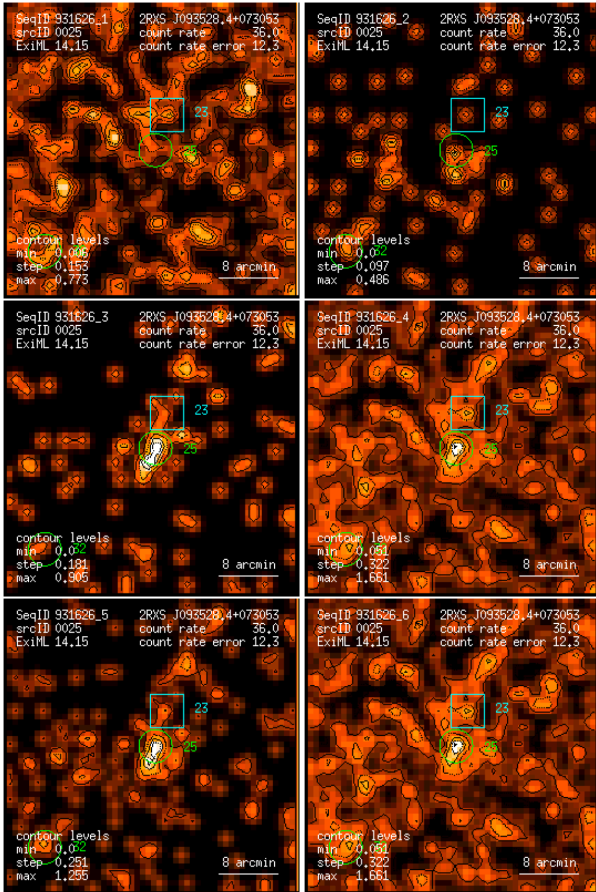
Figure 25: RASS 931626: detection 0025: band rate images, Gaussian filter: (1) PSPC channels 11 – 41, (2) 52 – 90, (3) 91 – 201, (4) 11 – 235, (5) 52 – 201, (6) 11 – 201. Broad band rates in counts/ks. Band rate contour levels in counts/ks/arcmin 2 .
