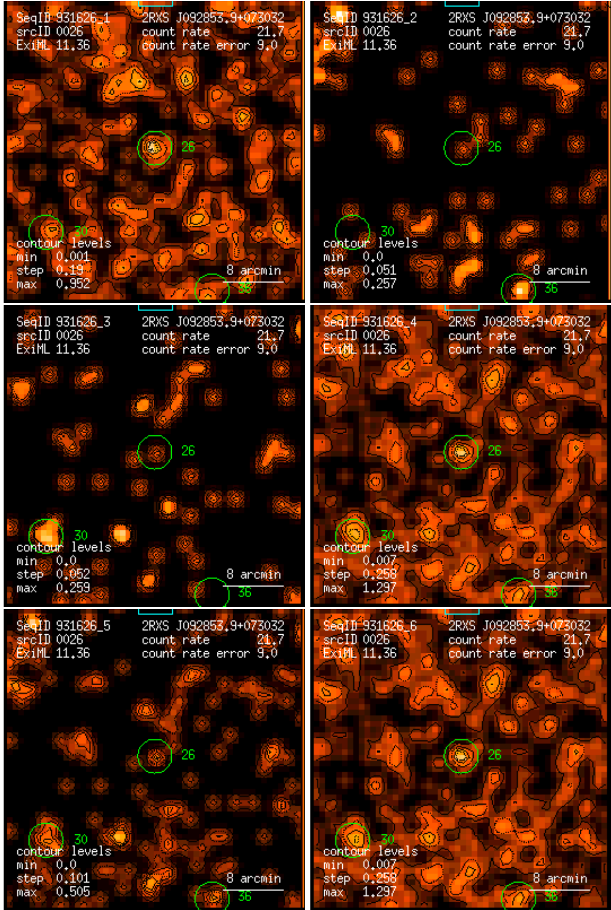
Figure 26: RASS 931626: detection 0026: band rate images, Gaussian filter: (1) PSPC channels 11 – 41, (2) 52 – 90, (3) 91 – 201, (4) 11 – 235, (5) 52 – 201, (6) 11 – 201. Broad band rates in counts/ks. Band rate contour levels in counts/ks/arcmin 2 .
