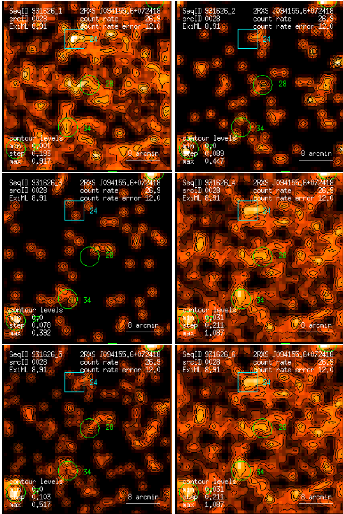
Figure 28: RASS 931626: detection 0028: band rate images, Gaussian filter: (1) PSPC channels 11 – 41, (2) 52 – 90, (3) 91 – 201, (4) 11 – 235, (5) 52 – 201, (6) 11 – 201. Broad band rates in counts/ks. Band rate contour levels in counts/ks/arcmin 2 .
