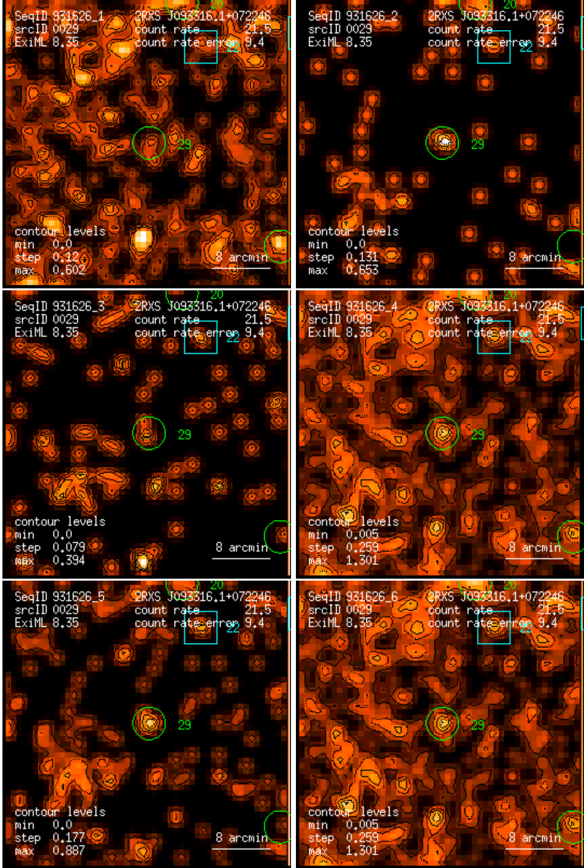
Figure 29: RASS 931626: detection 0029: band rate images, Gaussian filter: (1) PSPC channels 11 – 41, (2) 52 – 90, (3) 91 – 201, (4) 11 – 235, (5) 52 – 201, (6) 11 – 201. Broad band rates in counts/ks. Band rate contour levels in counts/ks/arcmin 2 .
