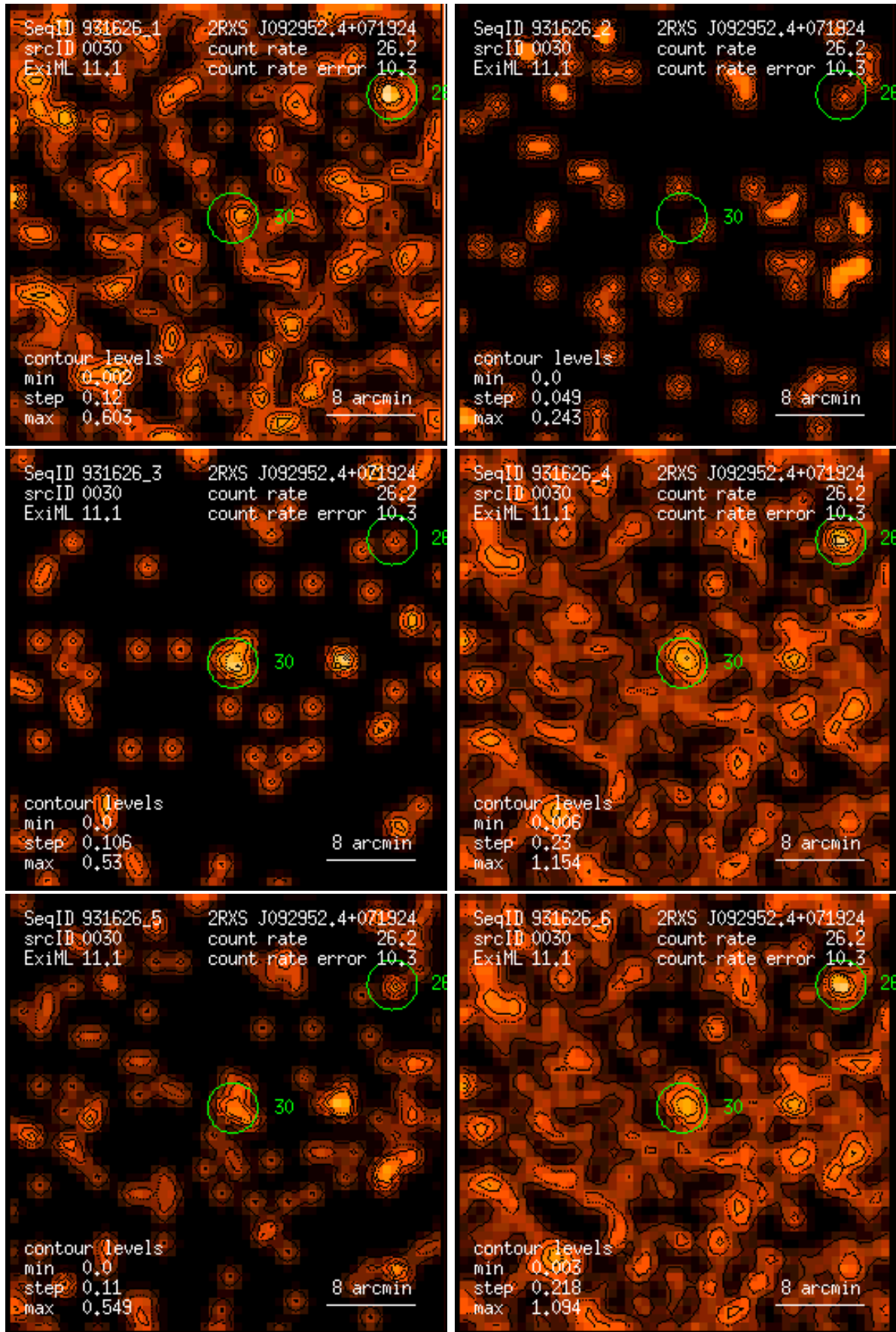
Figure 30: RASS 931626: detection 0030: band rate images, Gaussian filter: (1) PSPC channels 11 – 41, (2) 52 – 90, (3) 91 – 201, (4) 11 – 235, (5) 52 – 201, (6) 11 – 201. Broad band rates in counts/ks. Band rate contour levels in counts/ks/arcmin 2 .
