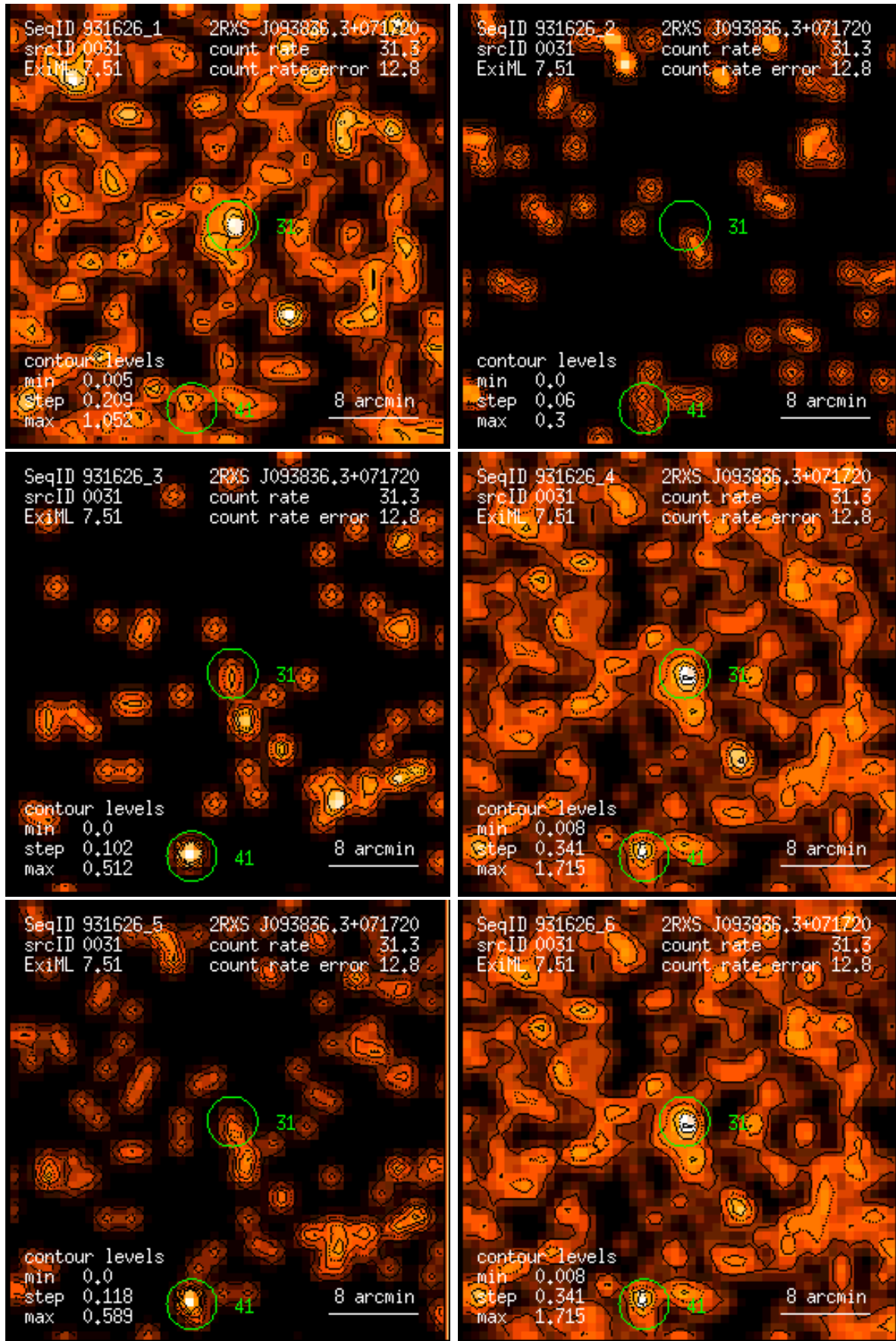
Figure 31: RASS 931626: detection 0031: band rate images, Gaussian filter: (1) PSPC channels 11 – 41, (2) 52 – 90, (3) 91 – 201, (4) 11 – 235, (5) 52 – 201, (6) 11 – 201. Broad band rates in counts/ks. Band rate contour levels in counts/ks/arcmin 2 .
