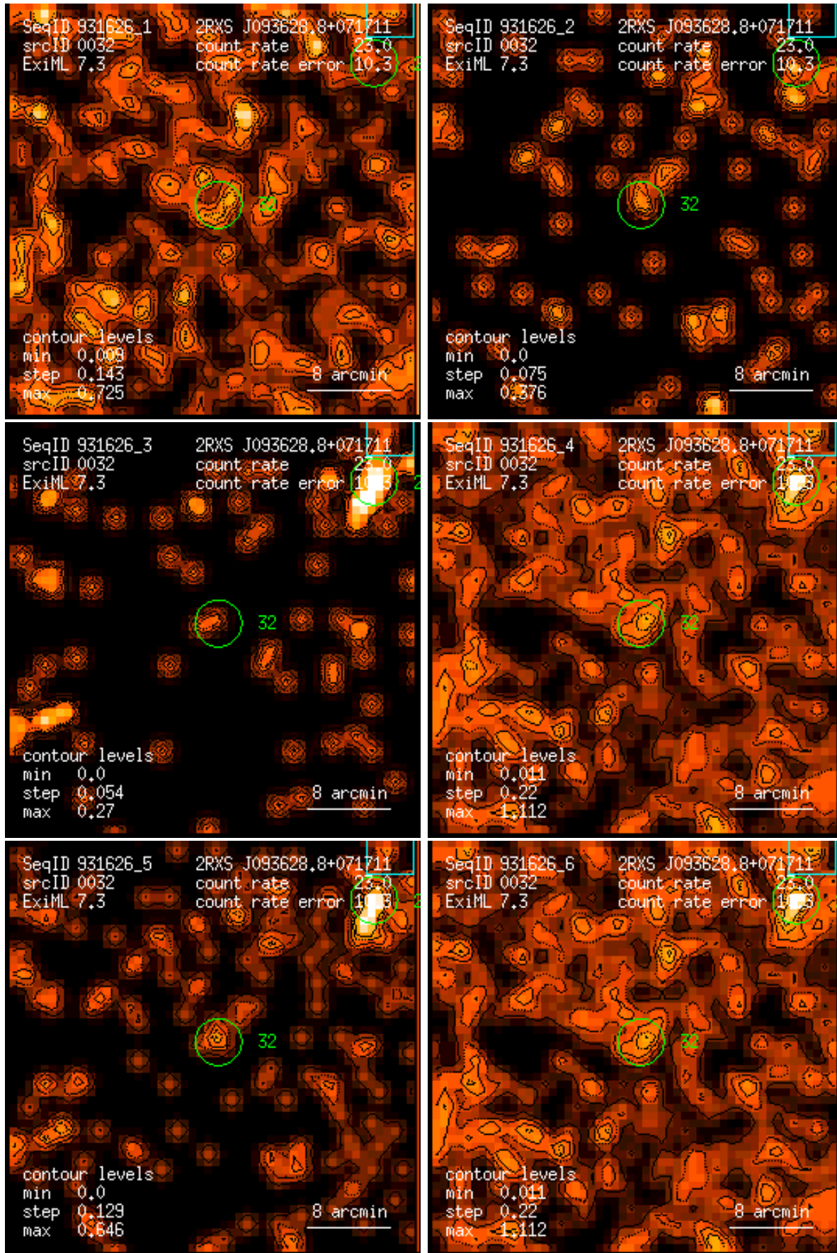
Figure 32: RASS 931626: detection 0032: band rate images, Gaussian filter: (1) PSPC channels 11 – 41, (2) 52 – 90, (3) 91 – 201, (4) 11 – 235, (5) 52 – 201, (6) 11 – 201. Broad band rates in counts/ks. Band rate contour levels in counts/ks/arcmin 2 .
