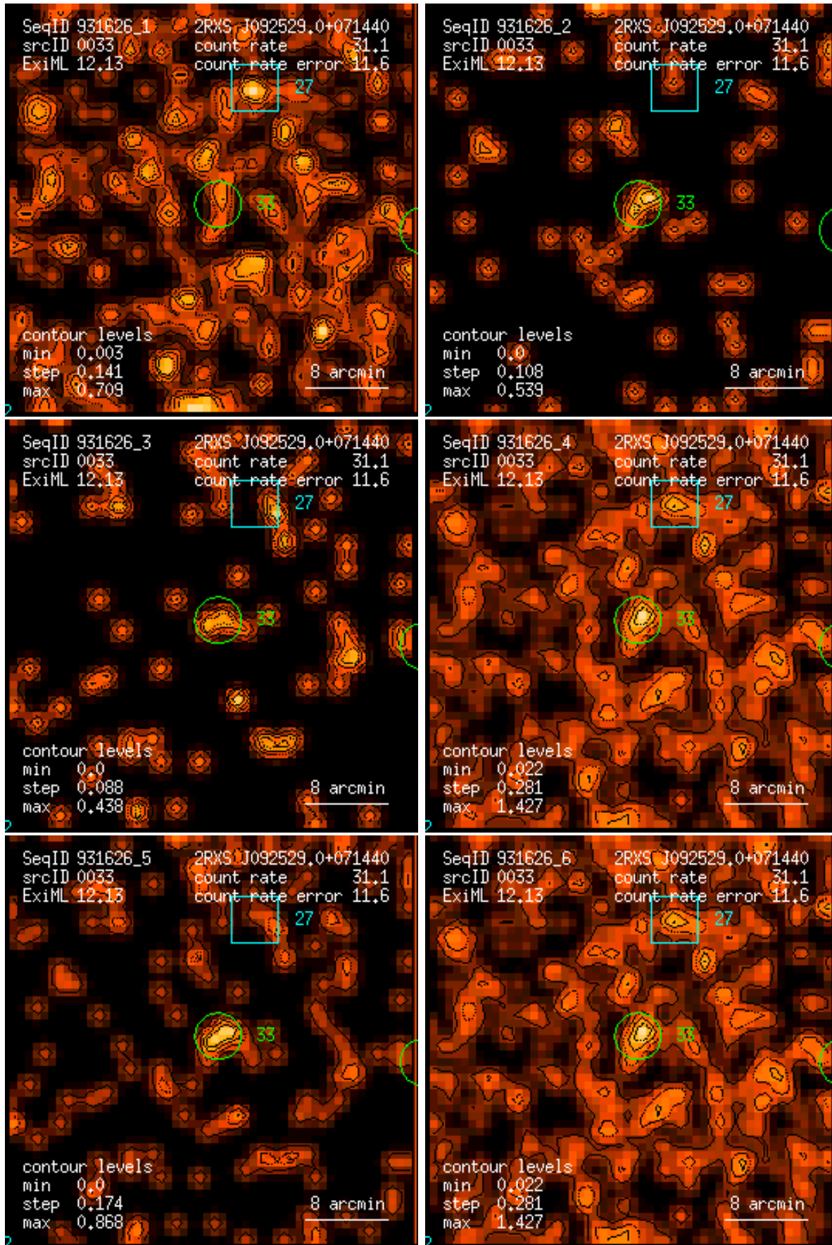
Figure 33: RASS 931626: detection 0033: band rate images, Gaussian filter: (1) PSPC channels 11 – 41, (2) 52 – 90, (3) 91 – 201, (4) 11 – 235, (5) 52 – 201, (6) 11 – 201. Broad band rates in counts/ks. Band rate contour levels in counts/ks/arcmin 2 .
