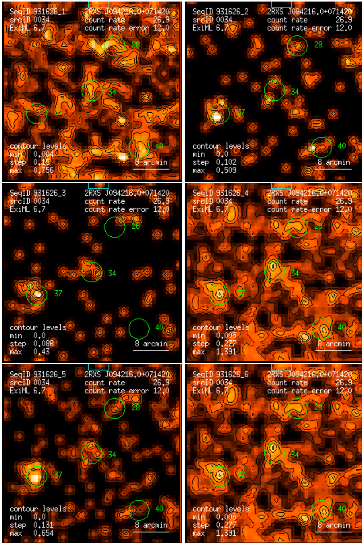
Figure 34: RASS 931626: detection 0034: band rate images, Gaussian filter: (1) PSPC channels 11 – 41, (2) 52 – 90, (3) 91 – 201, (4) 11 – 235, (5) 52 – 201, (6) 11 – 201. Broad band rates in counts/ks. Band rate contour levels in counts/ks/arcmin 2 .
