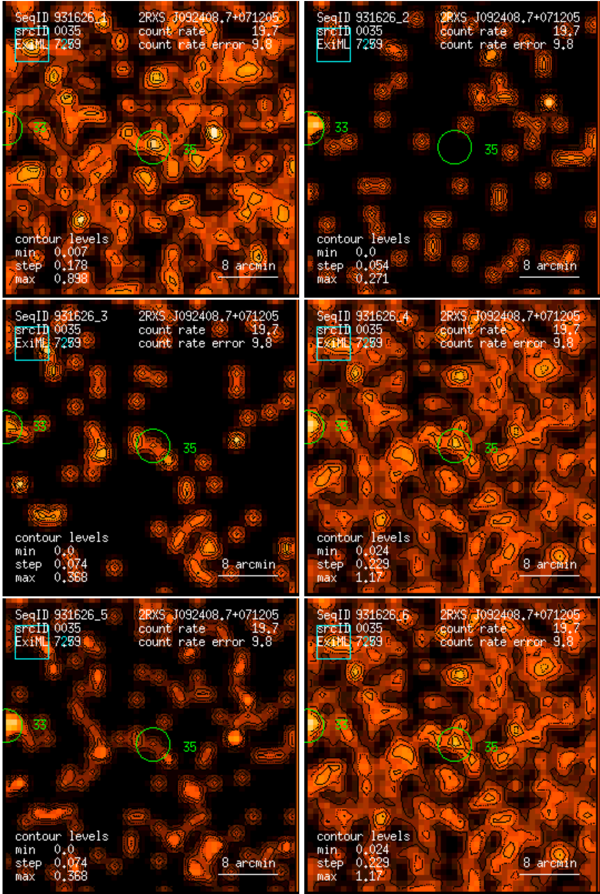
Figure 35: RASS 931626: detection 0035: band rate images, Gaussian filter: (1) PSPC channels 11 – 41, (2) 52 – 90, (3) 91 – 201, (4) 11 – 235, (5) 52 – 201, (6) 11 – 201. Broad band rates in counts/ks. Band rate contour levels in counts/ks/arcmin 2 .
