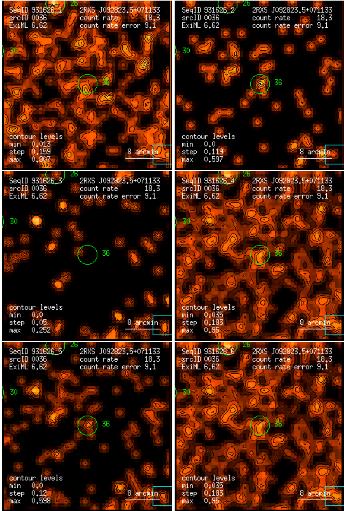
Figure 36: RASS 931626: detection 0036: band rate images, Gaussian filter: (1) PSPC channels 11 – 41, (2) 52 – 90, (3) 91 – 201, (4) 11 – 235, (5) 52 – 201, (6) 11 – 201. Broad band rates in counts/ks. Band rate contour levels in counts/ks/arcmin 2 .
