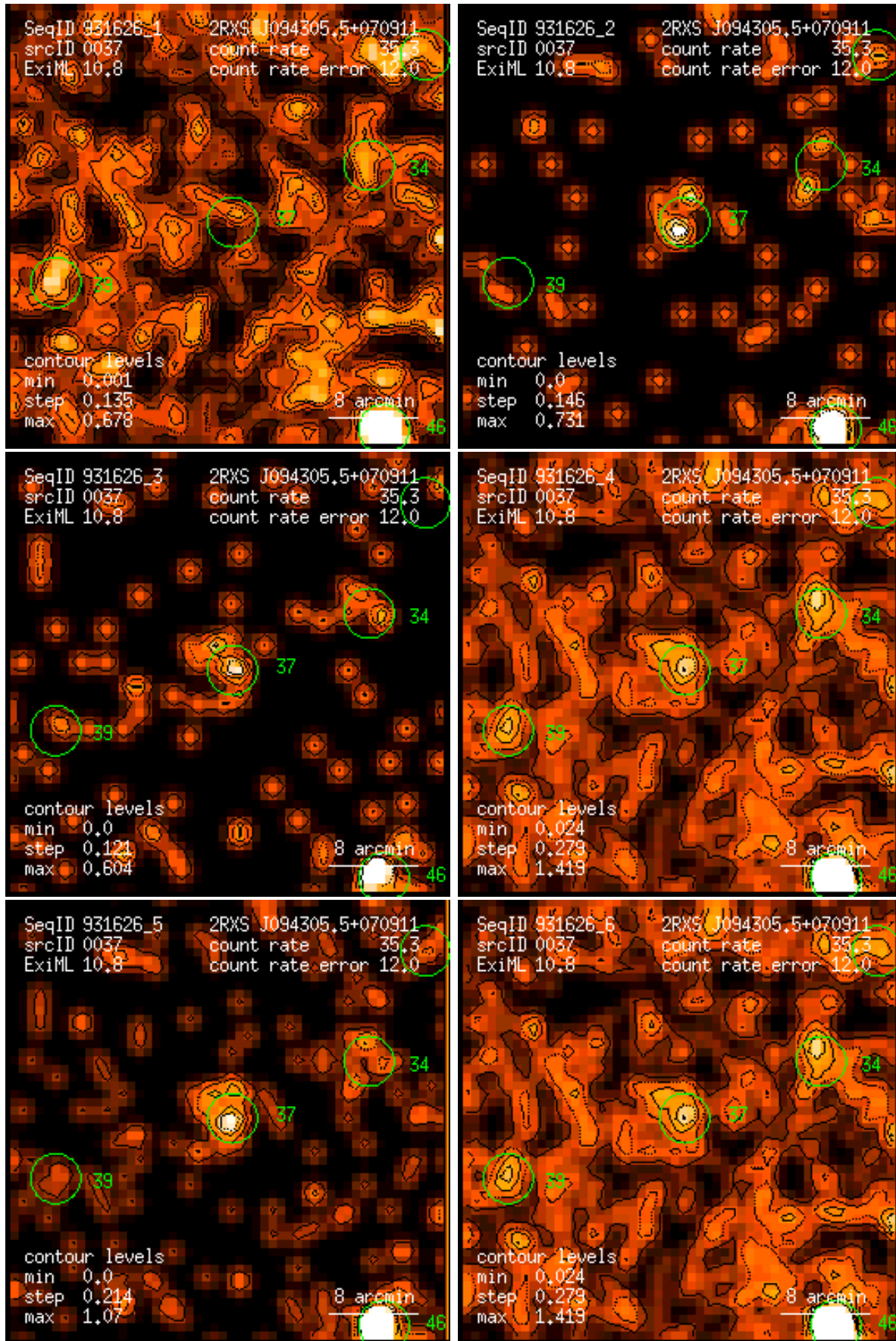
Figure 37: RASS 931626: detection 0037: band rate images, Gaussian filter: (1) PSPC channels 11 – 41, (2) 52 – 90, (3) 91 – 201, (4) 11 – 235, (5) 52 – 201, (6) 11 – 201. Broad band rates in counts/ks. Band rate contour levels in counts/ks/arcmin 2 .
