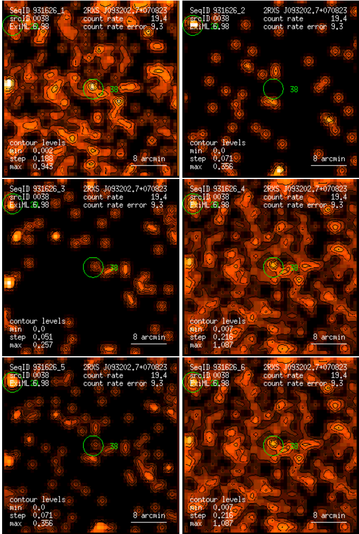
Figure 38: RASS 931626: detection 0038: band rate images, Gaussian filter: (1) PSPC channels 11 – 41, (2) 52 – 90, (3) 91 – 201, (4) 11 – 235, (5) 52 – 201, (6) 11 – 201. Broad band rates in counts/ks. Band rate contour levels in counts/ks/arcmin 2 .
