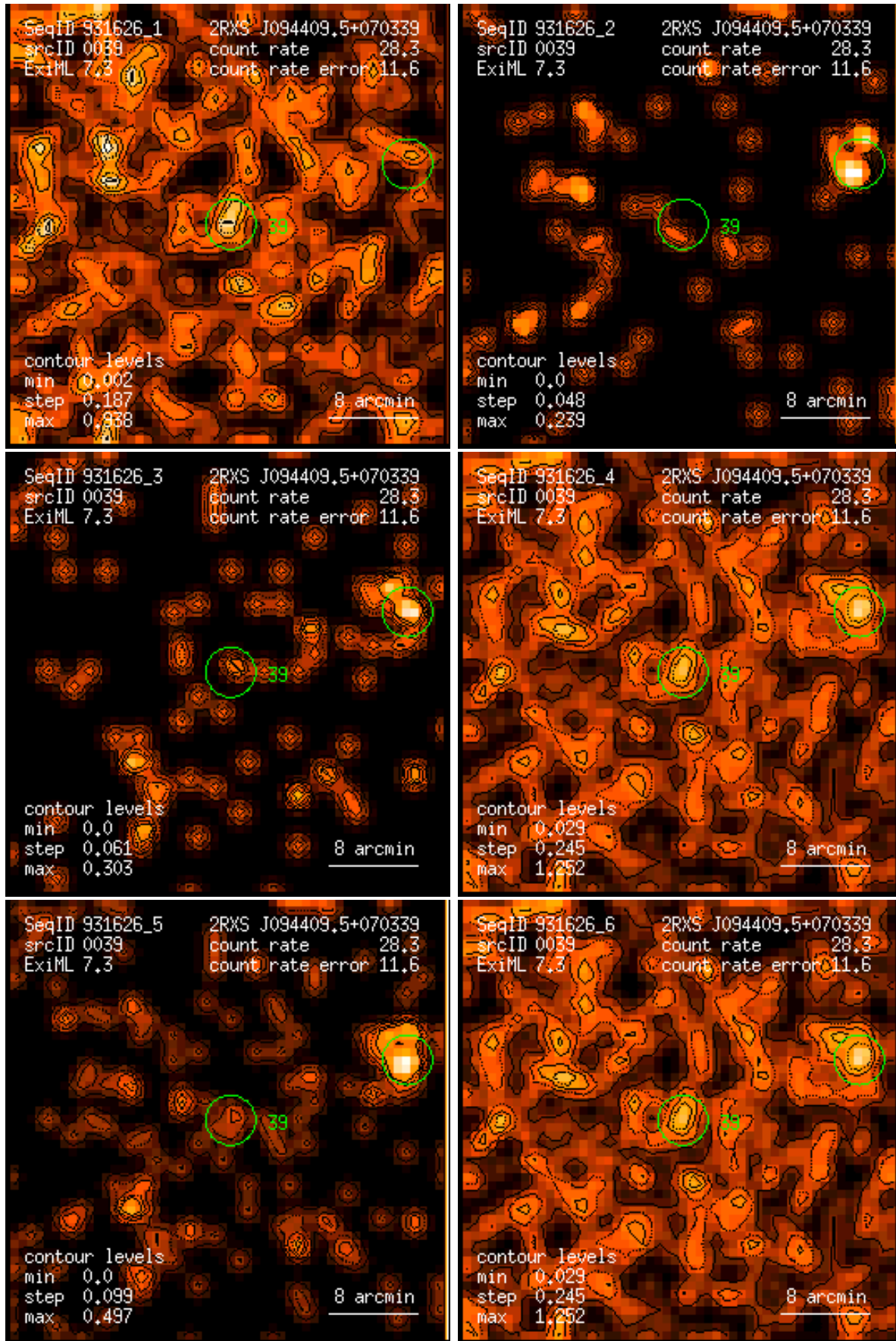
Figure 39: RASS 931626: detection 0039: band rate images, Gaussian filter: (1) PSPC channels 11 – 41, (2) 52 – 90, (3) 91 – 201, (4) 11 – 235, (5) 52 – 201, (6) 11 – 201. Broad band rates in counts/ks. Band rate contour levels in counts/ks/arcmin 2 .
