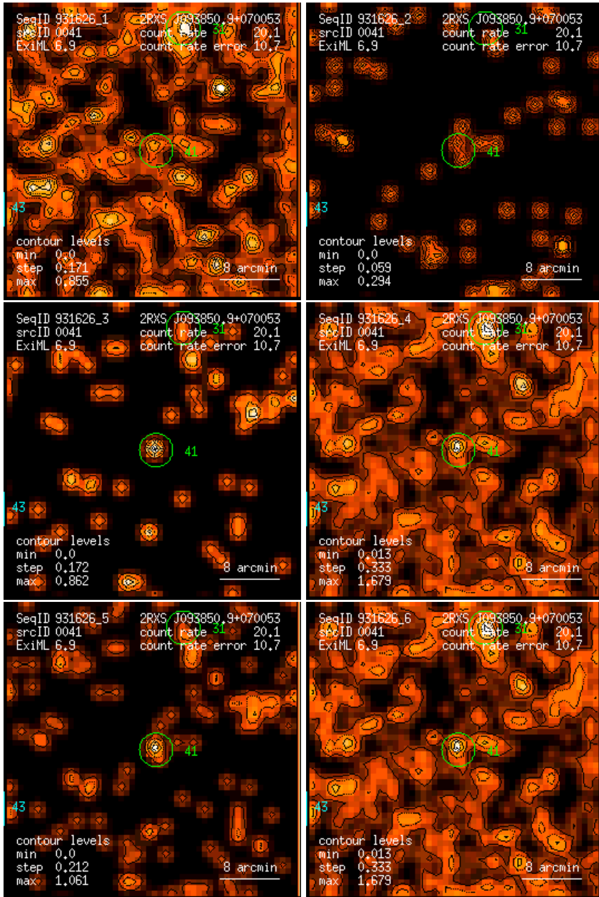
Figure 41: RASS 931626: detection 0041: band rate images, Gaussian filter: (1) PSPC channels 11 – 41, (2) 52 – 90, (3) 91 – 201, (4) 11 – 235, (5) 52 – 201, (6) 11 – 201. Broad band rates in counts/ks. Band rate contour levels in counts/ks/arcmin 2 .
