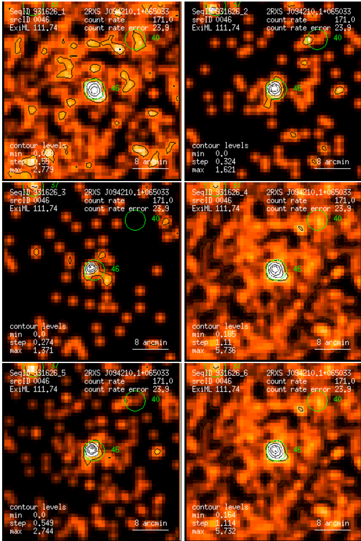
Figure 46: RASS 931626: detection 0046: band rate images, Gaussian filter: (1) PSPC channels 11 – 41, (2) 52 – 90, (3) 91 – 201, (4) 11 – 235, (5) 52 – 201, (6) 11 – 201. Broad band rates in counts/ks. Band rate contour levels in counts/ks/arcmin 2 .
