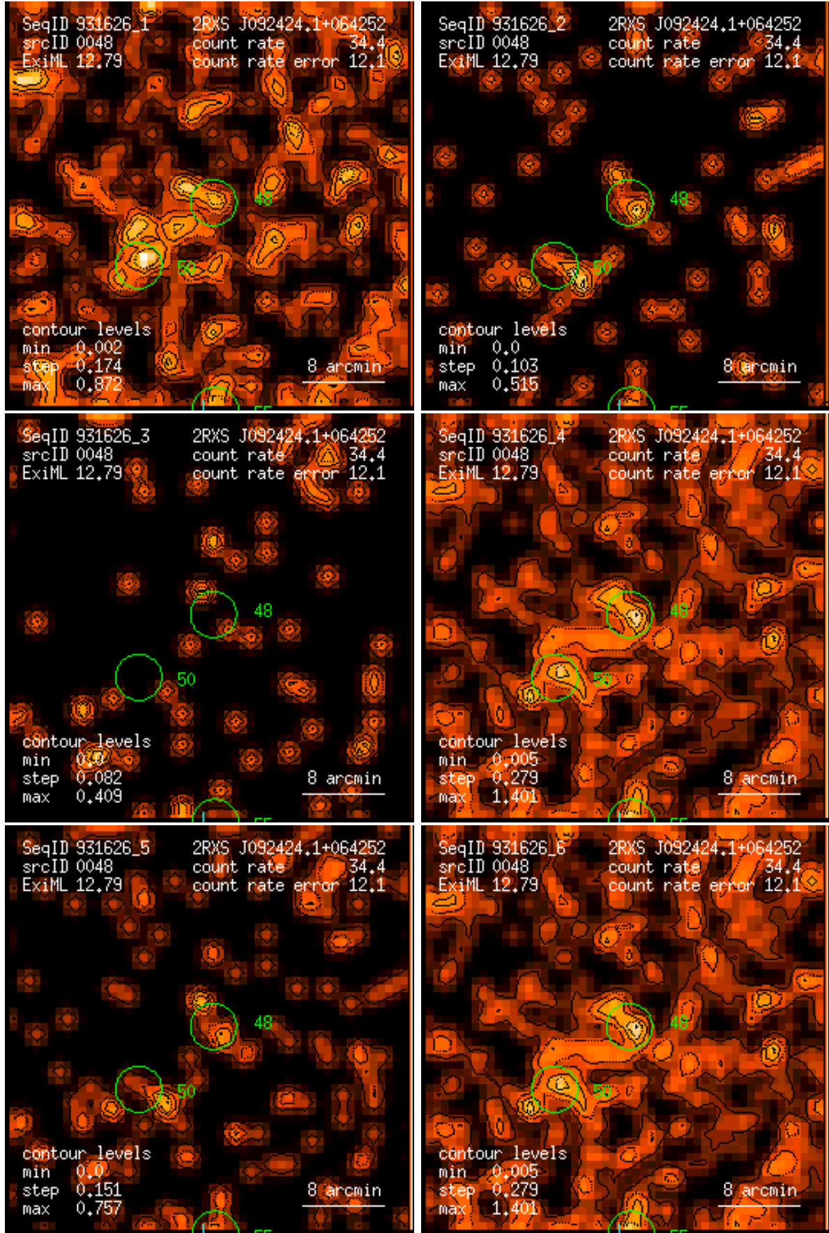
Figure 48: RASS 931626: detection 0048: band rate images, Gaussian filter: (1) PSPC channels 11 – 41, (2) 52 – 90, (3) 91 – 201, (4) 11 – 235, (5) 52 – 201, (6) 11 – 201. Broad band rates in counts/ks. Band rate contour levels in counts/ks/arcmin 2 .
