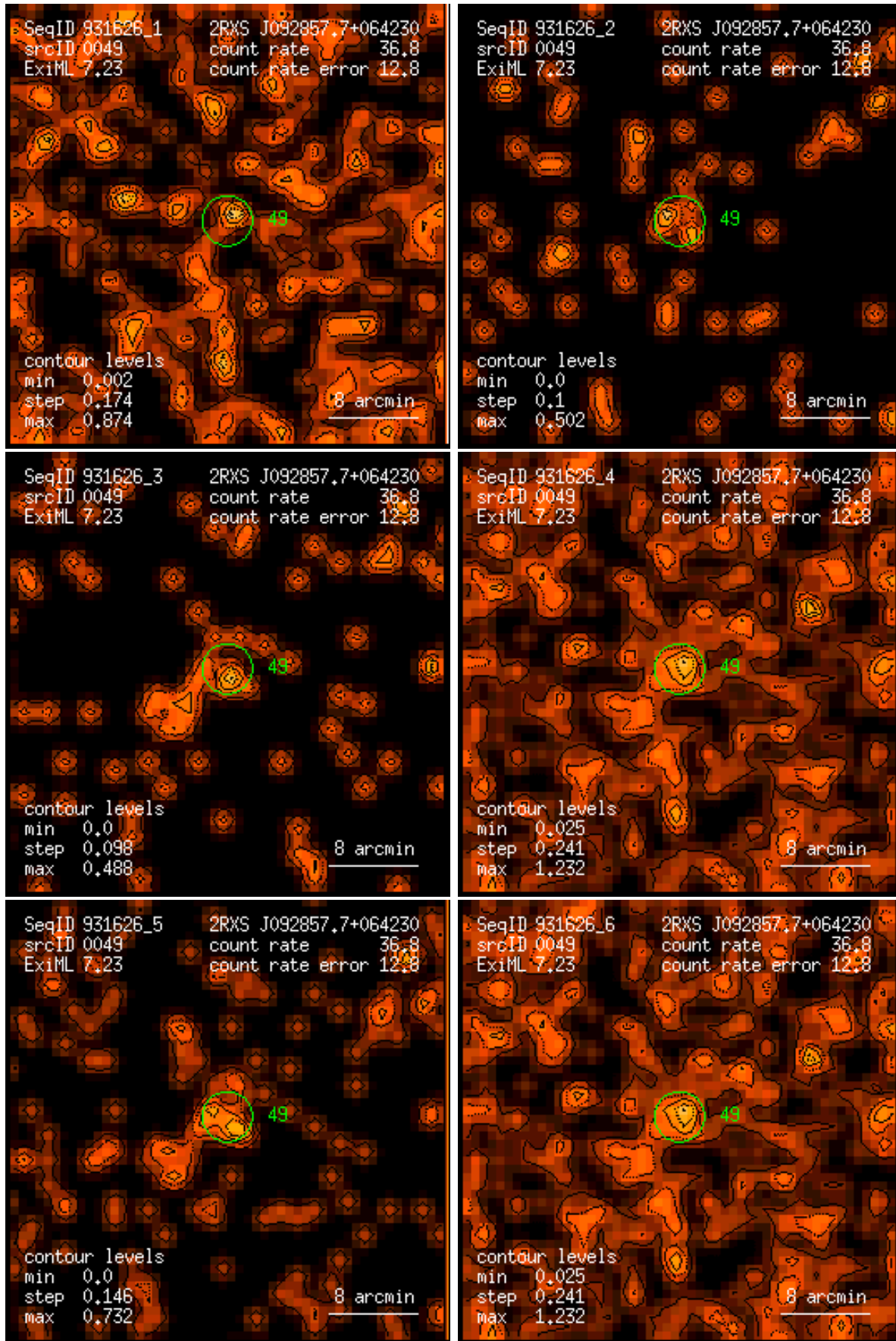
Figure 49: RASS 931626: detection 0049: band rate images, Gaussian filter: (1) PSPC channels 11 – 41, (2) 52 – 90, (3) 91 – 201, (4) 11 – 235, (5) 52 – 201, (6) 11 – 201. Broad band rates in counts/ks. Band rate contour levels in counts/ks/arcmin 2 .
