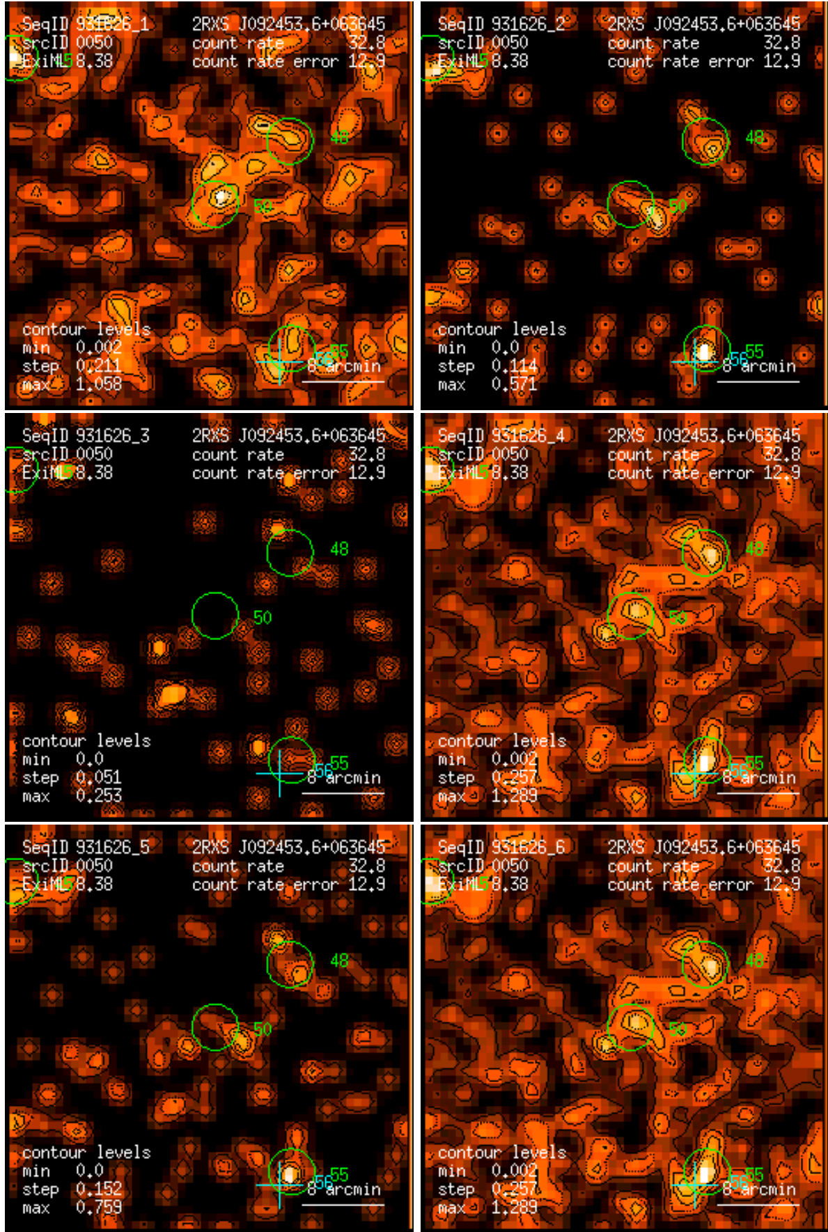
Figure 50: RASS 931626: detection 0050: band rate images, Gaussian filter: (1) PSPC channels 11 – 41, (2) 52 – 90, (3) 91 – 201, (4) 11 – 235, (5) 52 – 201, (6) 11 – 201. Broad band rates in counts/ks. Band rate contour levels in counts/ks/arcmin 2 .
