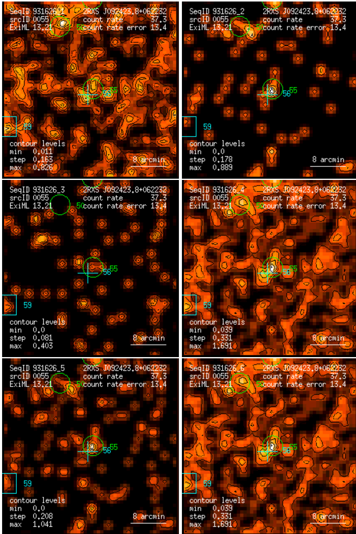
Figure 55: RASS 931626: detection 0055: band rate images, Gaussian filter: (1) PSPC channels 11 – 41, (2) 52 – 90, (3) 91 – 201, (4) 11 – 235, (5) 52 – 201, (6) 11 – 201. Broad band rates in counts/ks. Band rate contour levels in counts/ks/arcmin 2 .
