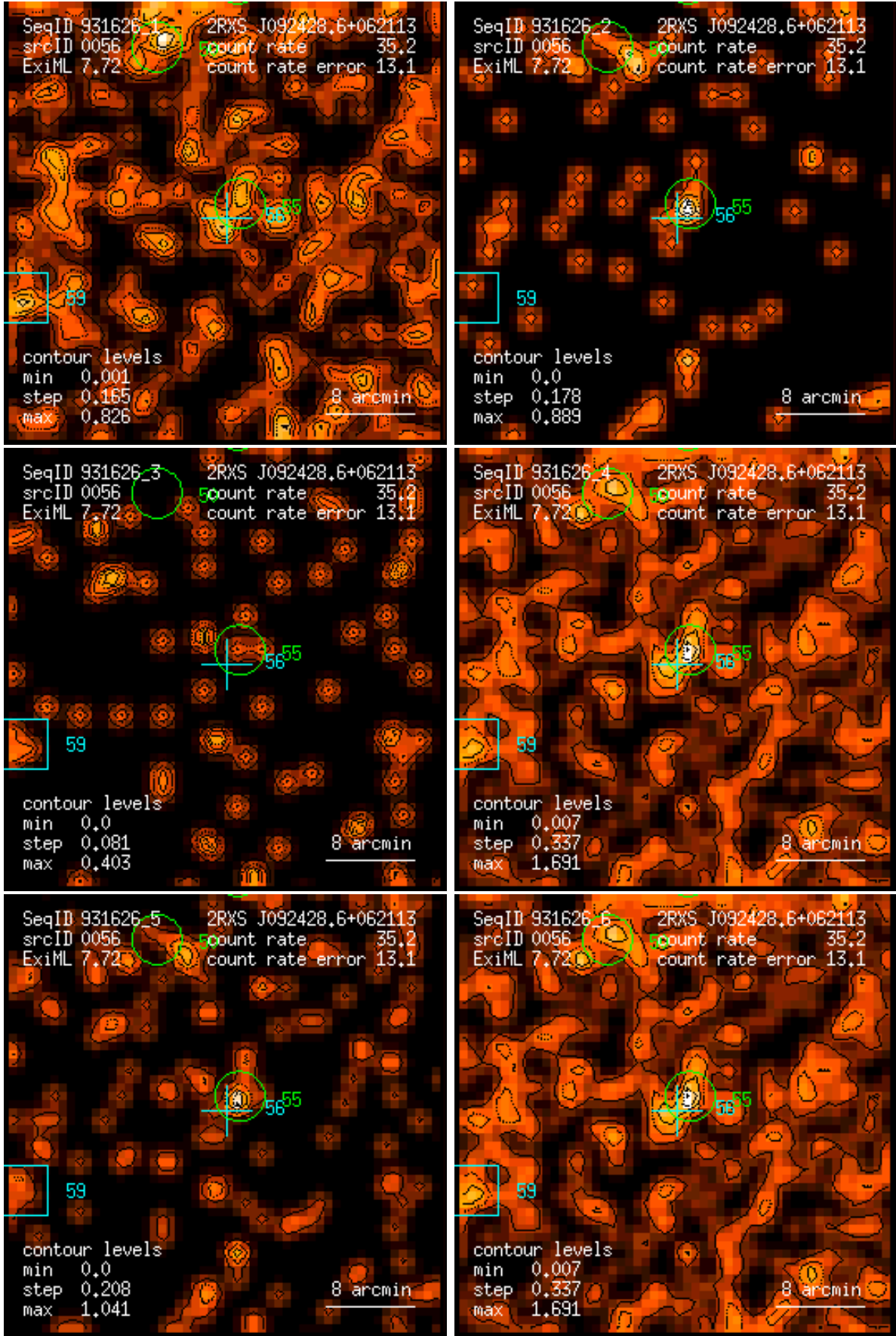
Figure 56: RASS 931626: detection 0056: band rate images, Gaussian filter: (1) PSPC channels 11 – 41, (2) 52 – 90, (3) 91 – 201, (4) 11 – 235, (5) 52 – 201, (6) 11 – 201. Broad band rates in counts/ks. Band rate contour levels in counts/ks/arcmin 2 .
