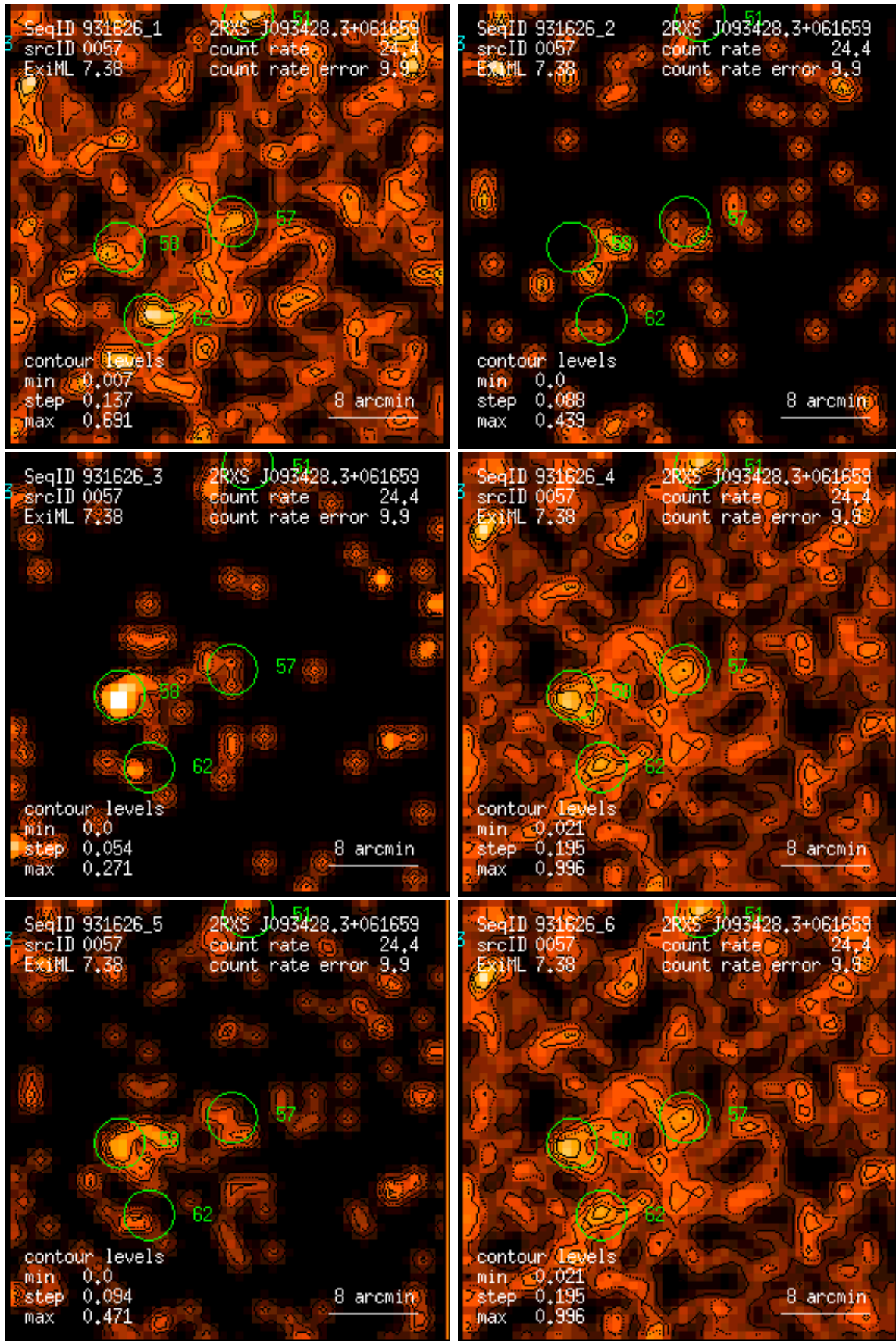
Figure 57: RASS 931626: detection 0057: band rate images, Gaussian filter: (1) PSPC channels 11 – 41, (2) 52 – 90, (3) 91 – 201, (4) 11 – 235, (5) 52 – 201, (6) 11 – 201. Broad band rates in counts/ks. Band rate contour levels in counts/ks/arcmin 2 .
