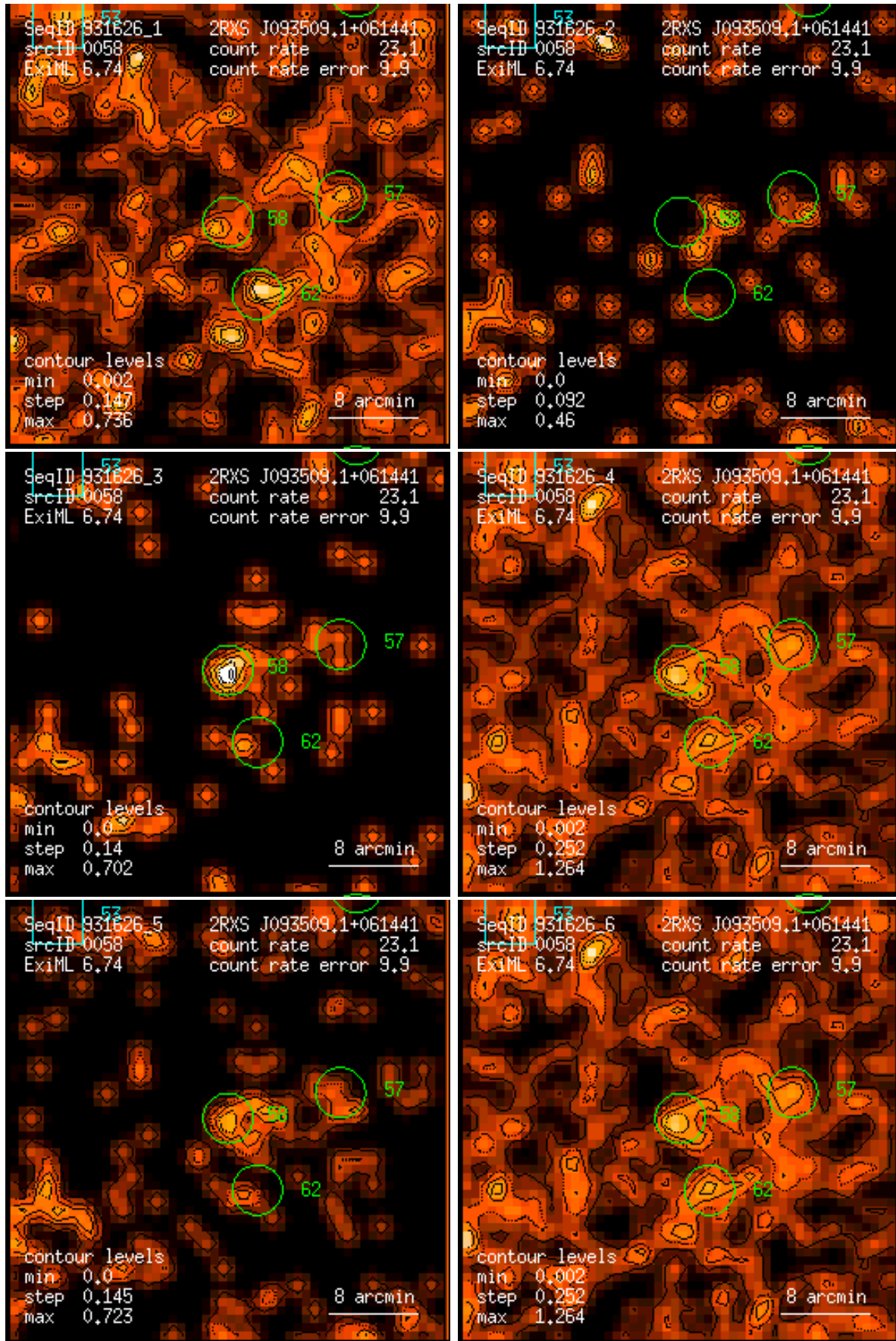
Figure 58: RASS 931626: detection 0058: band rate images, Gaussian filter: (1) PSPC channels 11 – 41, (2) 52 – 90, (3) 91 – 201, (4) 11 – 235, (5) 52 – 201, (6) 11 – 201. Broad band rates in counts/ks. Band rate contour levels in counts/ks/arcmin 2 .
