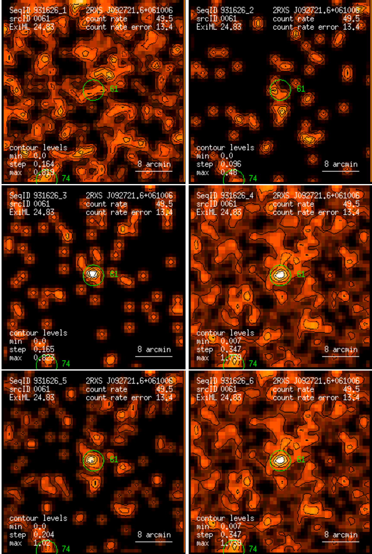
Figure 61: RASS 931626: detection 0061: band rate images, Gaussian filter: (1) PSPC channels 11 – 41, (2) 52 – 90, (3) 91 – 201, (4) 11 – 235, (5) 52 – 201, (6) 11 – 201. Broad band rates in counts/ks. Band rate contour levels in counts/ks/arcmin 2 .
