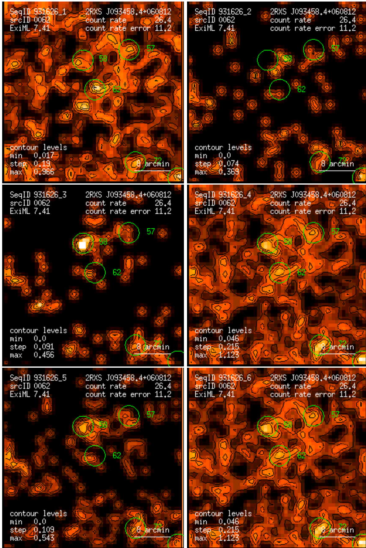
Figure 62: RASS 931626: detection 0062: band rate images, Gaussian filter: (1) PSPC channels 11 – 41, (2) 52 – 90, (3) 91 – 201, (4) 11 – 235, (5) 52 – 201, (6) 11 – 201. Broad band rates in counts/ks. Band rate contour levels in counts/ks/arcmin 2 .
