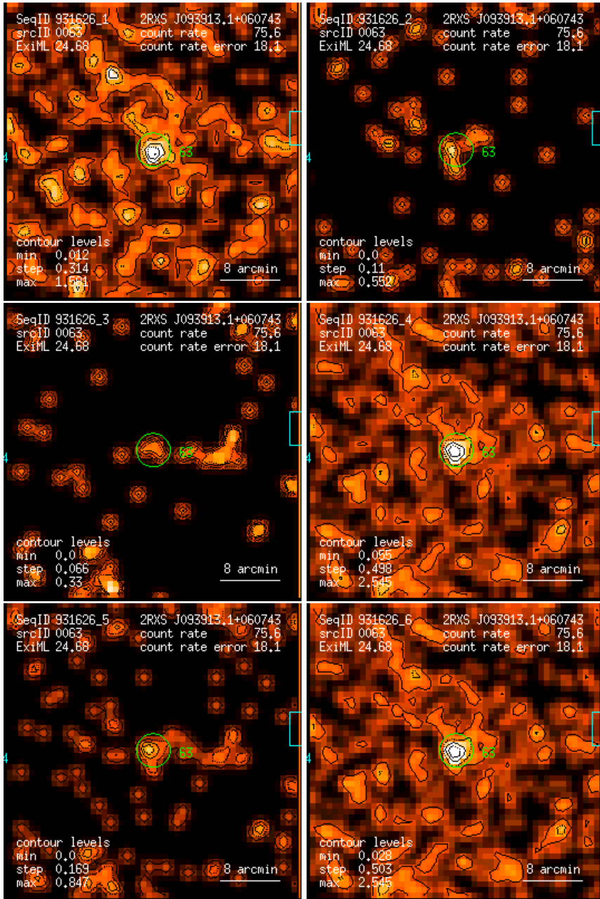
Figure 63: RASS 931626: detection 0063: band rate images, Gaussian filter: (1) PSPC channels 11 – 41, (2) 52 – 90, (3) 91 – 201, (4) 11 – 235, (5) 52 – 201, (6) 11 – 201. Broad band rates in counts/ks. Band rate contour levels in counts/ks/arcmin 2 .
