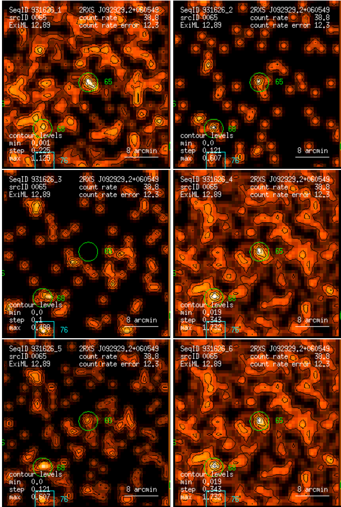
Figure 65: RASS 931626: detection 0065: band rate images, Gaussian filter: (1) PSPC channels 11 – 41, (2) 52 – 90, (3) 91 – 201, (4) 11 – 235, (5) 52 – 201, (6) 11 – 201. Broad band rates in counts/ks. Band rate contour levels in counts/ks/arcmin 2 .
