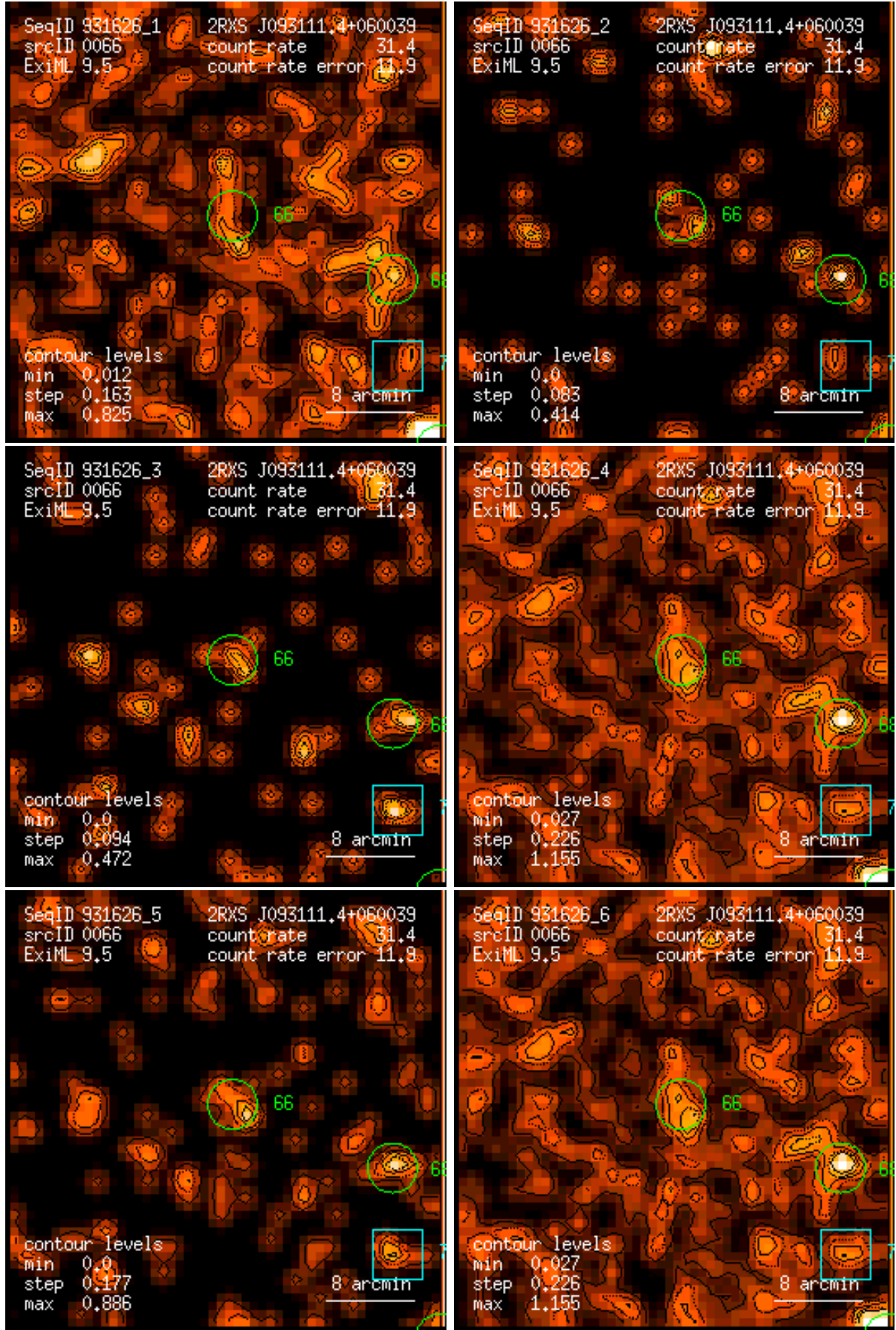
Figure 66: RASS 931626: detection 0066: band rate images, Gaussian filter: (1) PSPC channels 11 – 41, (2) 52 – 90, (3) 91 – 201, (4) 11 – 235, (5) 52 – 201, (6) 11 – 201. Broad band rates in counts/ks. Band rate contour levels in counts/ks/arcmin 2 .
