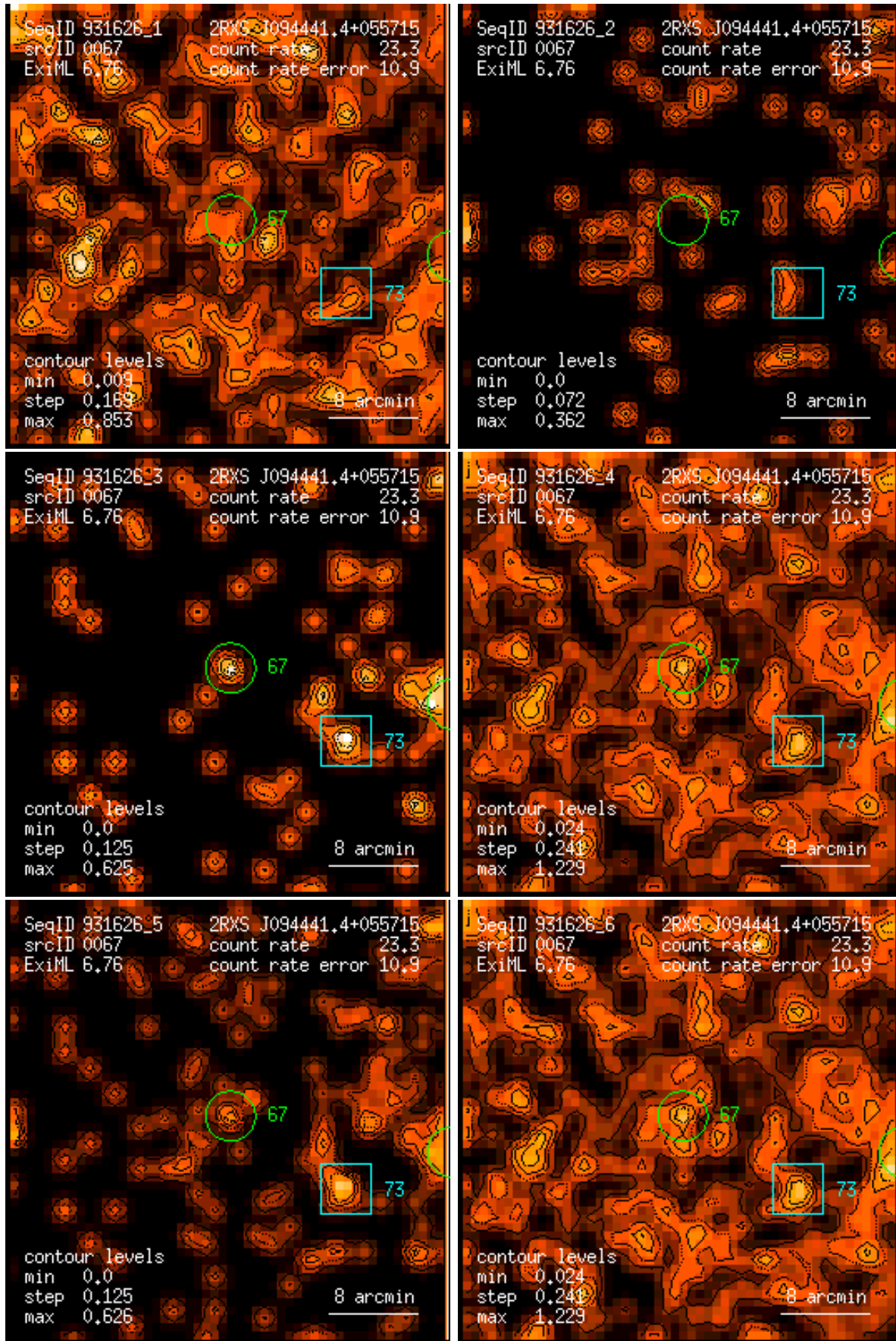
Figure 67: RASS 931626: detection 0067: band rate images, Gaussian filter: (1) PSPC channels 11 – 41, (2) 52 – 90, (3) 91 – 201, (4) 11 – 235, (5) 52 – 201, (6) 11 – 201. Broad band rates in counts/ks. Band rate contour levels in counts/ks/arcmin 2 .
