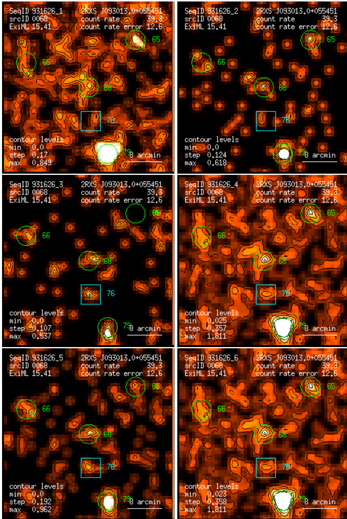
Figure 68: RASS 931626: detection 0068: band rate images, Gaussian filter: (1) PSPC channels 11 – 41, (2) 52 – 90, (3) 91 – 201, (4) 11 – 235, (5) 52 – 201, (6) 11 – 201. Broad band rates in counts/ks. Band rate contour levels in counts/ks/arcmin 2 .
