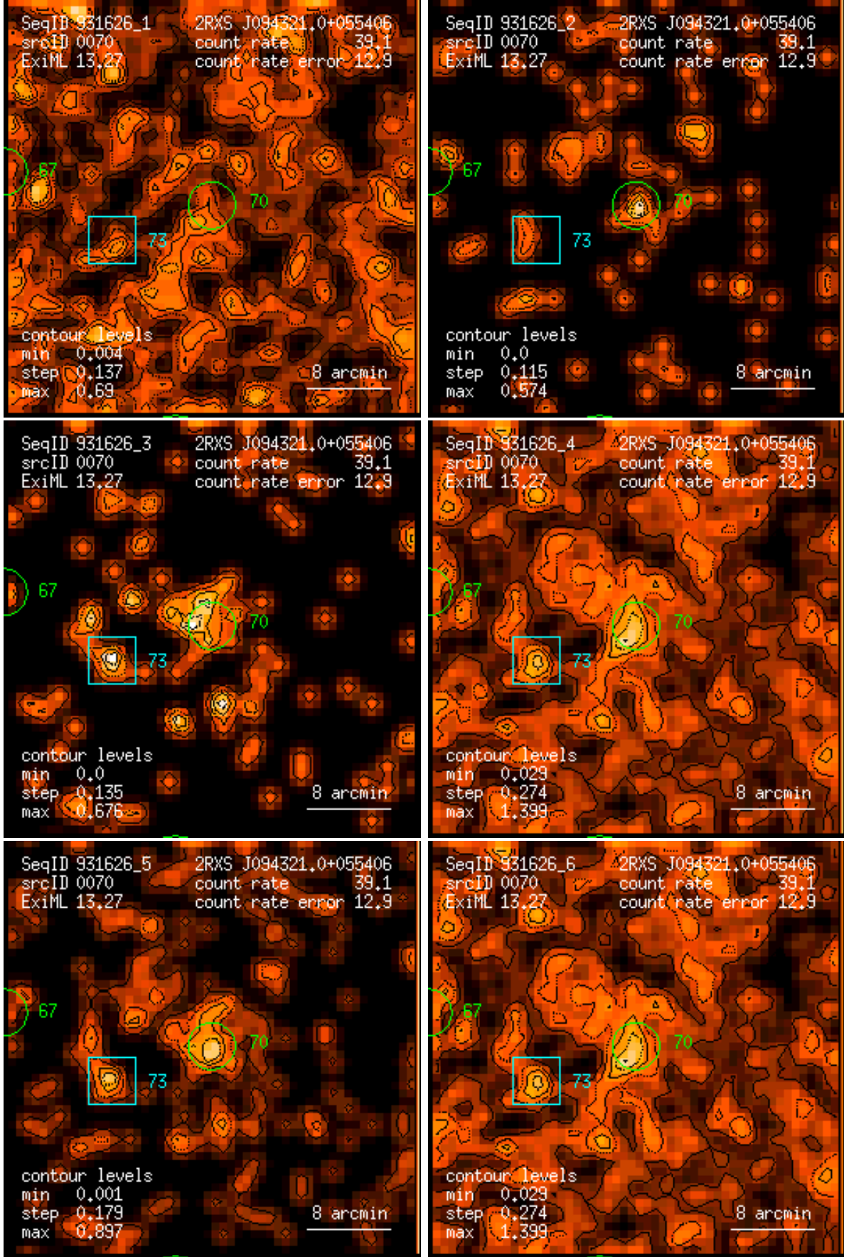
Figure 70: RASS 931626: detection 0070: band rate images, Gaussian filter: (1) PSPC channels 11 – 41, (2) 52 – 90, (3) 91 – 201, (4) 11 – 235, (5) 52 – 201, (6) 11 – 201. Broad band rates in counts/ks. Band rate contour levels in counts/ks/arcmin 2 .
