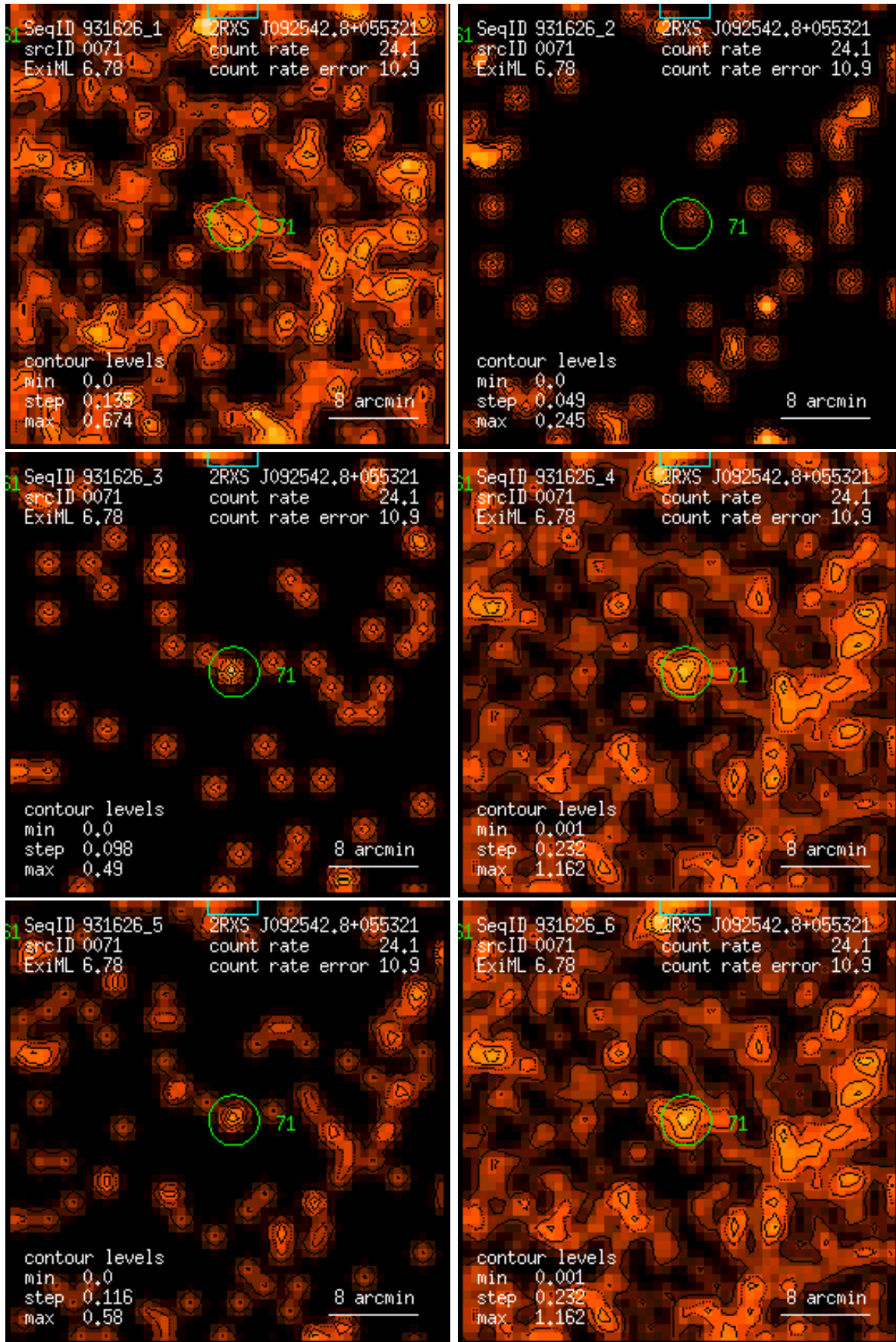
Figure 71: RASS 931626: detection 0071: band rate images, Gaussian filter: (1) PSPC channels 11 – 41, (2) 52 – 90, (3) 91 – 201, (4) 11 – 235, (5) 52 – 201, (6) 11 – 201. Broad band rates in counts/ks. Band rate contour levels in counts/ks/arcmin 2 .
