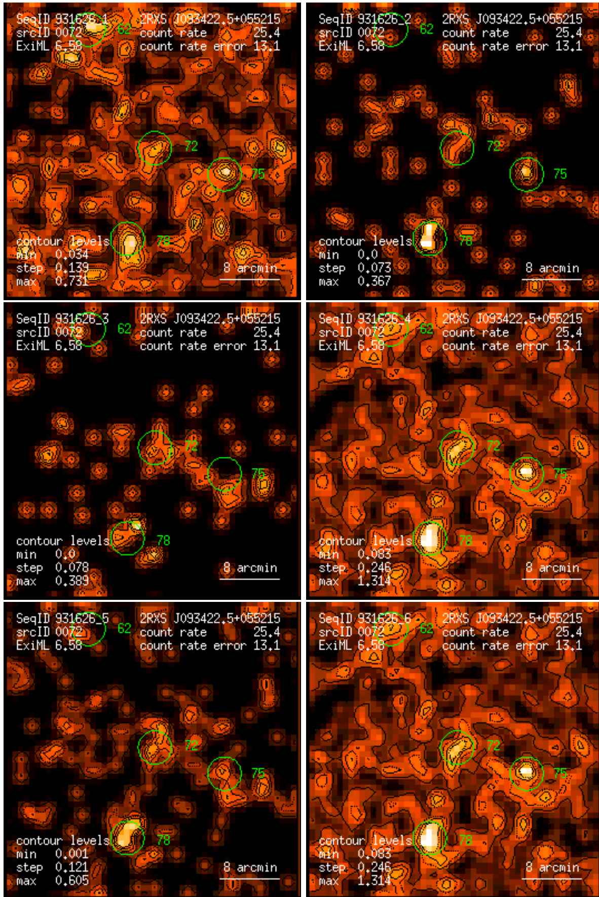
Figure 72: RASS 931626: detection 0072: band rate images, Gaussian filter: (1) PSPC channels 11 – 41, (2) 52 – 90, (3) 91 – 201, (4) 11 – 235, (5) 52 – 201, (6) 11 – 201. Broad band rates in counts/ks. Band rate contour levels in counts/ks/arcmin 2 .
