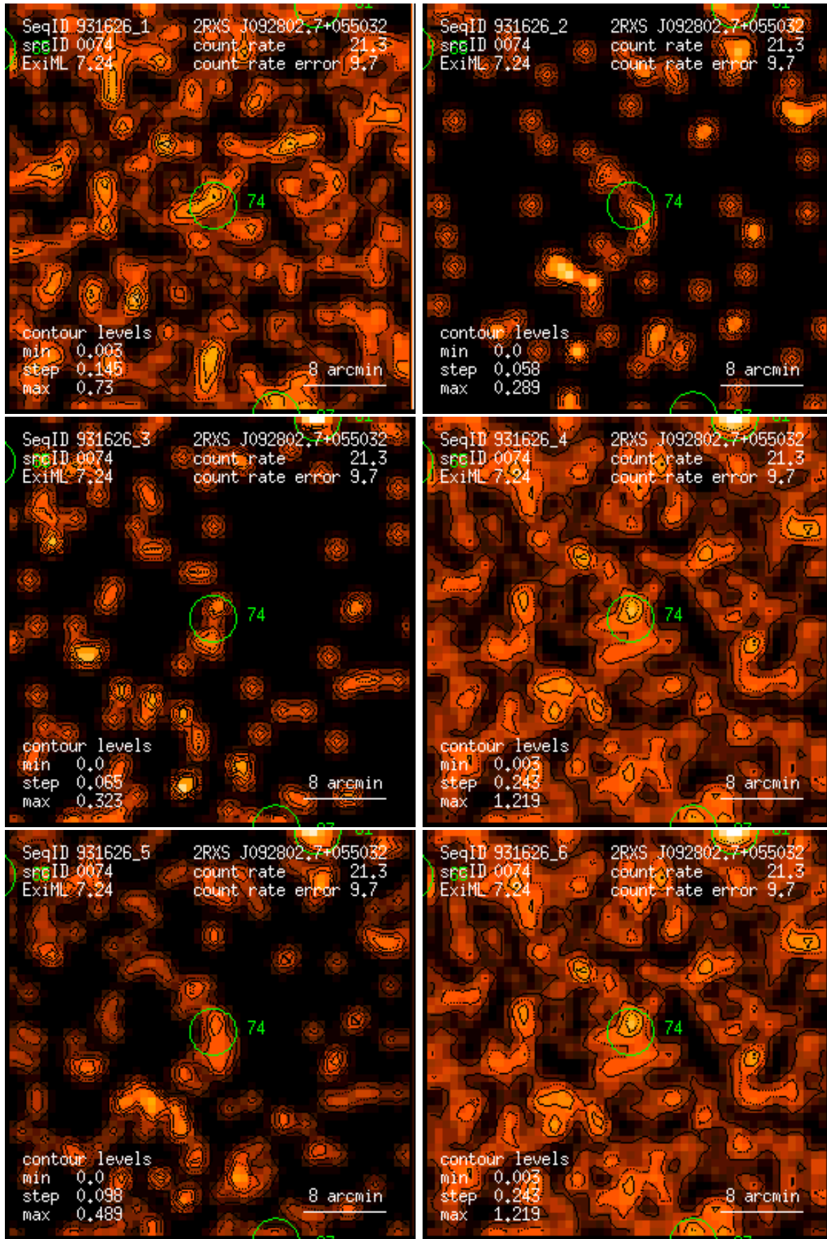
Figure 74: RASS 931626: detection 0074: band rate images, Gaussian filter: (1) PSPC channels 11 – 41, (2) 52 – 90, (3) 91 – 201, (4) 11 – 235, (5) 52 – 201, (6) 11 – 201. Broad band rates in counts/ks. Band rate contour levels in counts/ks/arcmin 2 .
