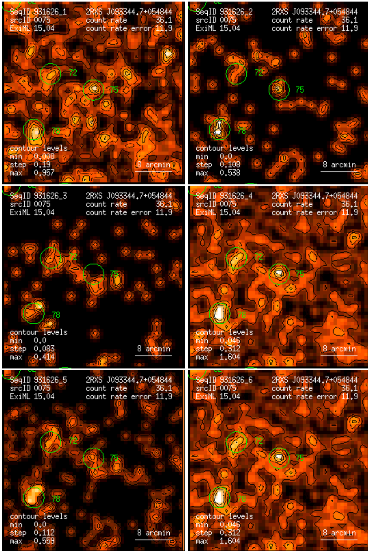
Figure 75: RASS 931626: detection 0075: band rate images, Gaussian filter: (1) PSPC channels 11 – 41, (2) 52 – 90, (3) 91 – 201, (4) 11 – 235, (5) 52 – 201, (6) 11 – 201. Broad band rates in counts/ks. Band rate contour levels in counts/ks/arcmin 2 .
