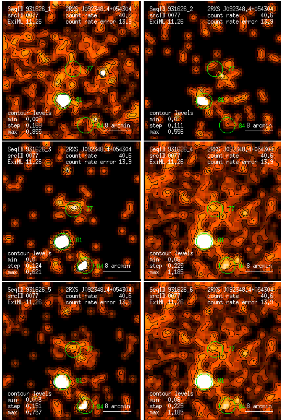
Figure 77: RASS 931626: detection 0077: band rate images, Gaussian filter: (1) PSPC channels 11 – 41, (2) 52 – 90, (3) 91 – 201, (4) 11 – 235, (5) 52 – 201, (6) 11 – 201. Broad band rates in counts/ks. Band rate contour levels in counts/ks/arcmin 2 .
