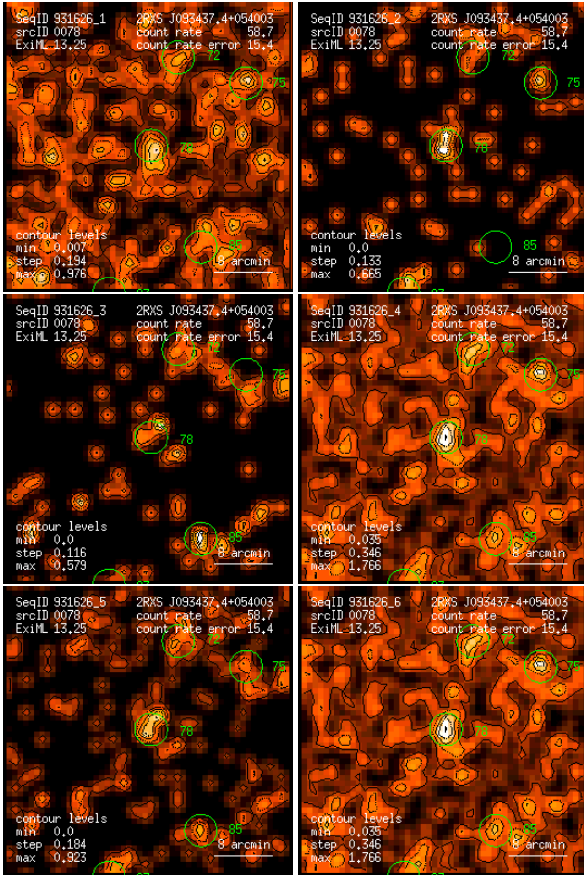
Figure 78: RASS 931626: detection 0078: band rate images, Gaussian filter: (1) PSPC channels 11 – 41, (2) 52 – 90, (3) 91 – 201, (4) 11 – 235, (5) 52 – 201, (6) 11 – 201. Broad band rates in counts/ks. Band rate contour levels in counts/ks/arcmin 2 .
