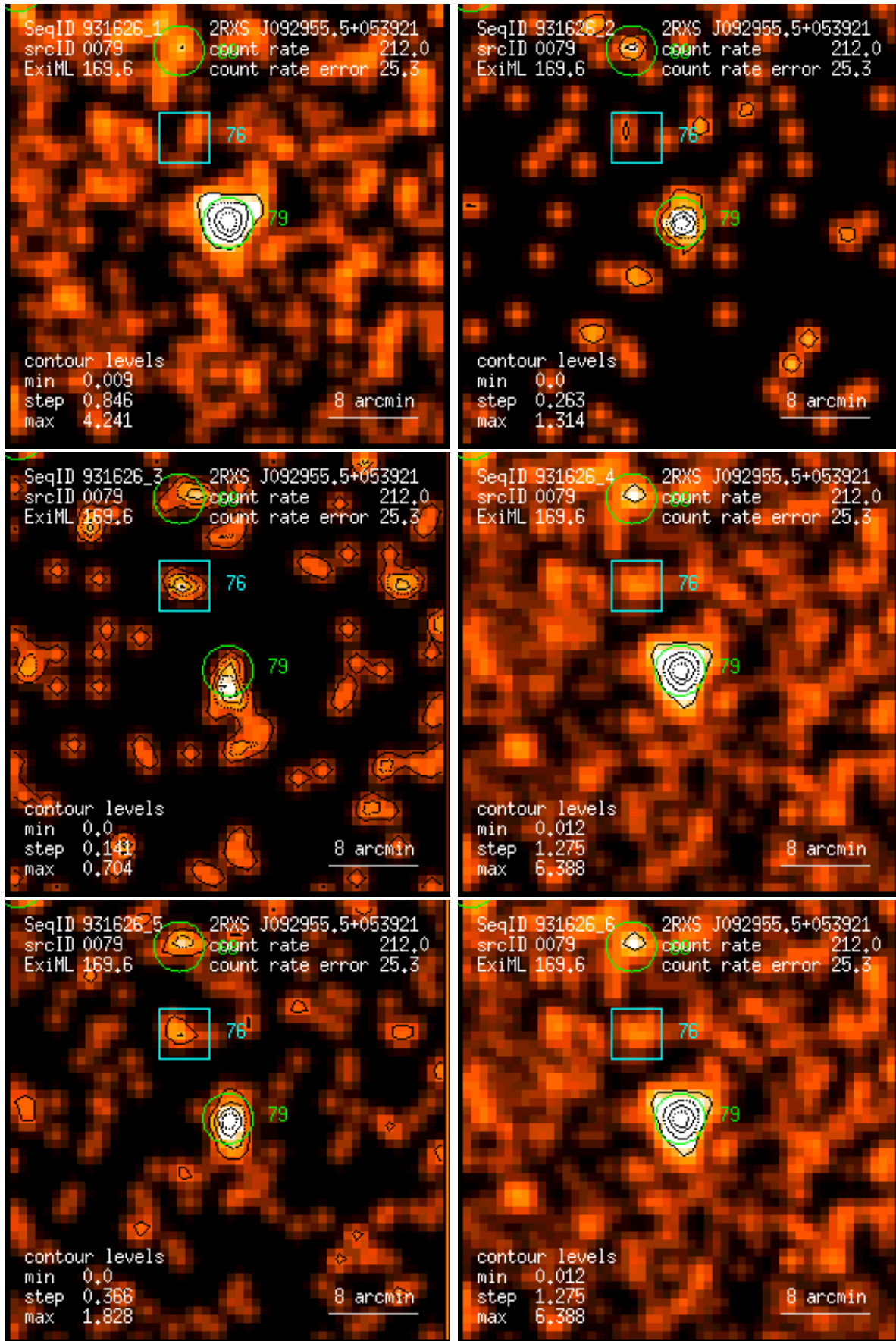
Figure 79: RASS 931626: detection 0079: band rate images, Gaussian filter: (1) PSPC channels 11 – 41, (2) 52 – 90, (3) 91 – 201, (4) 11 – 235, (5) 52 – 201, (6) 11 – 201. Broad band rates in counts/ks. Band rate contour levels in counts/ks/arcmin 2 .
