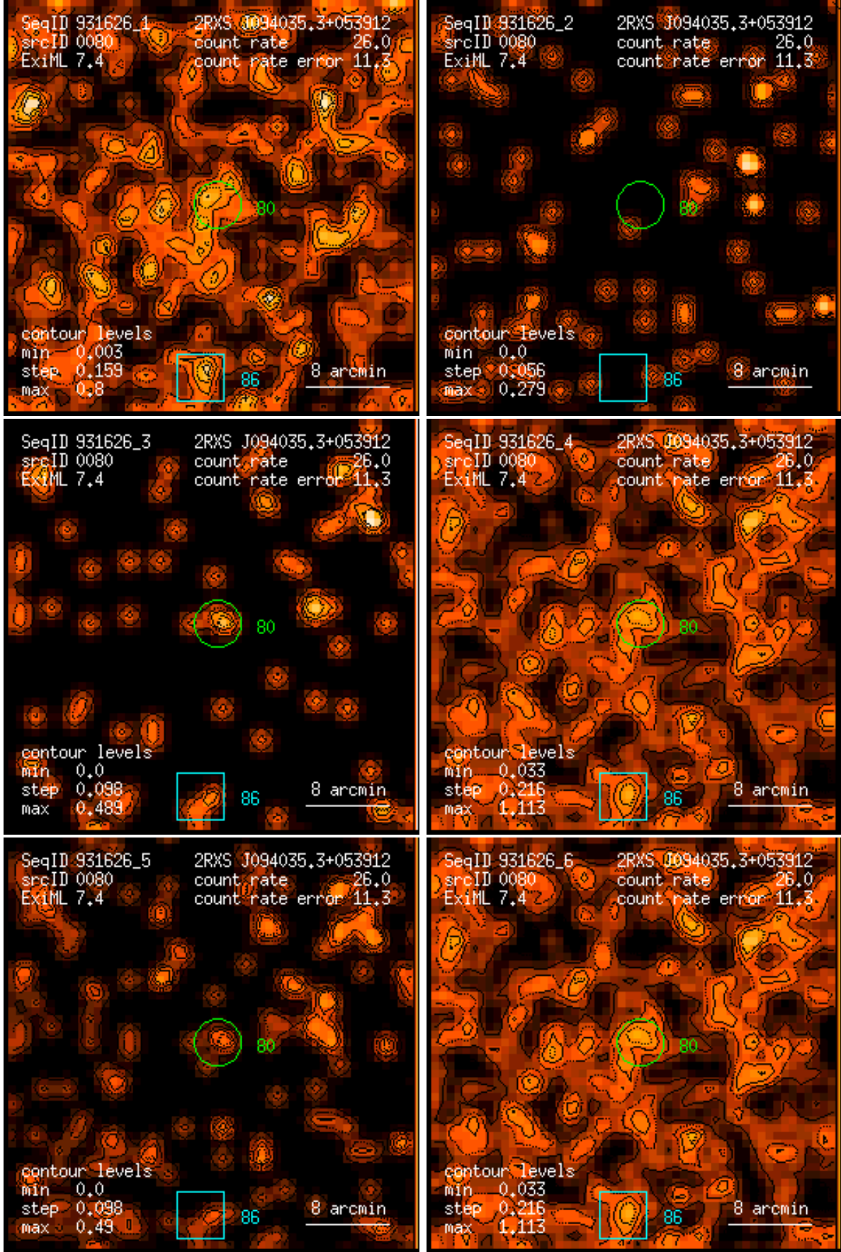
Figure 80: RASS 931626: detection 0080: band rate images, Gaussian filter: (1) PSPC channels 11 – 41, (2) 52 – 90, (3) 91 – 201, (4) 11 – 235, (5) 52 – 201, (6) 11 – 201. Broad band rates in counts/ks. Band rate contour levels in counts/ks/arcmin 2 .
