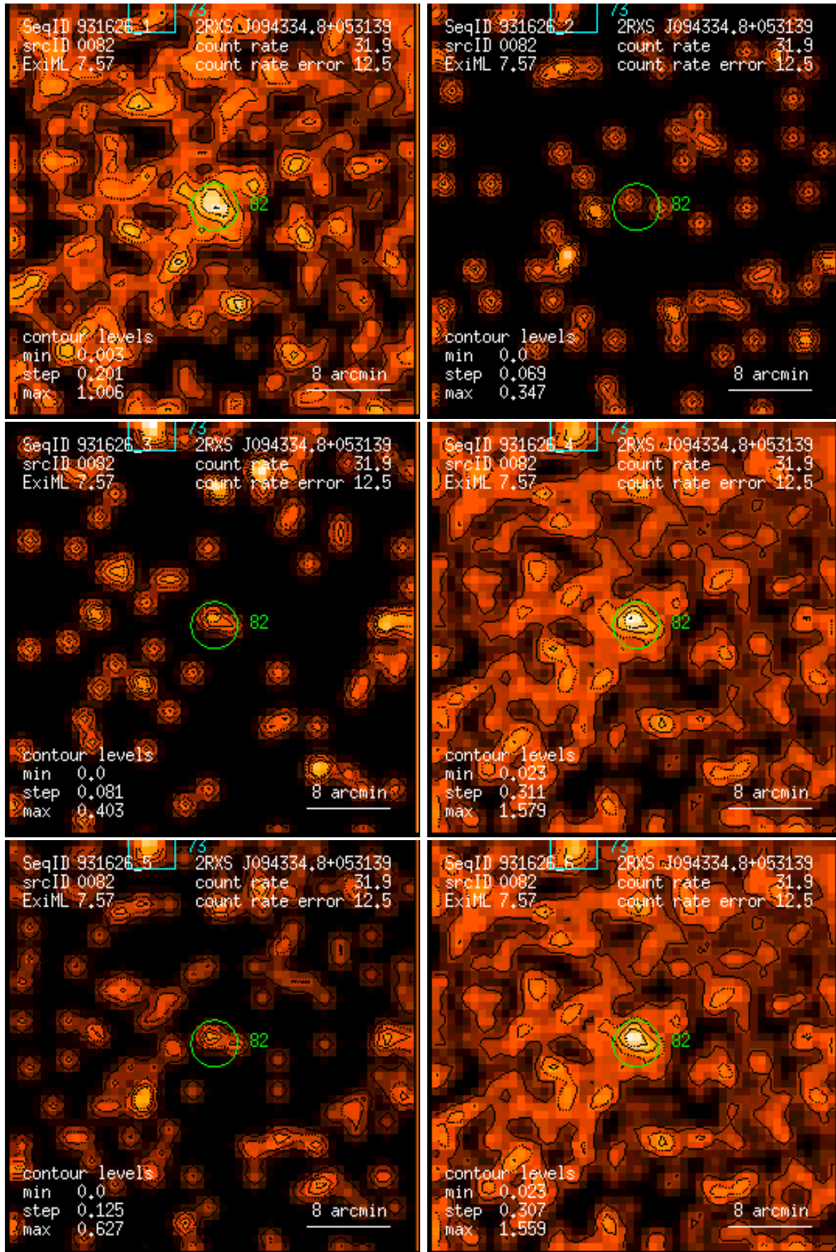
Figure 82: RASS 931626: detection 0082: band rate images, Gaussian filter: (1) PSPC channels 11 – 41, (2) 52 – 90, (3) 91 – 201, (4) 11 – 235, (5) 52 – 201, (6) 11 – 201. Broad band rates in counts/ks. Band rate contour levels in counts/ks/arcmin 2 .
