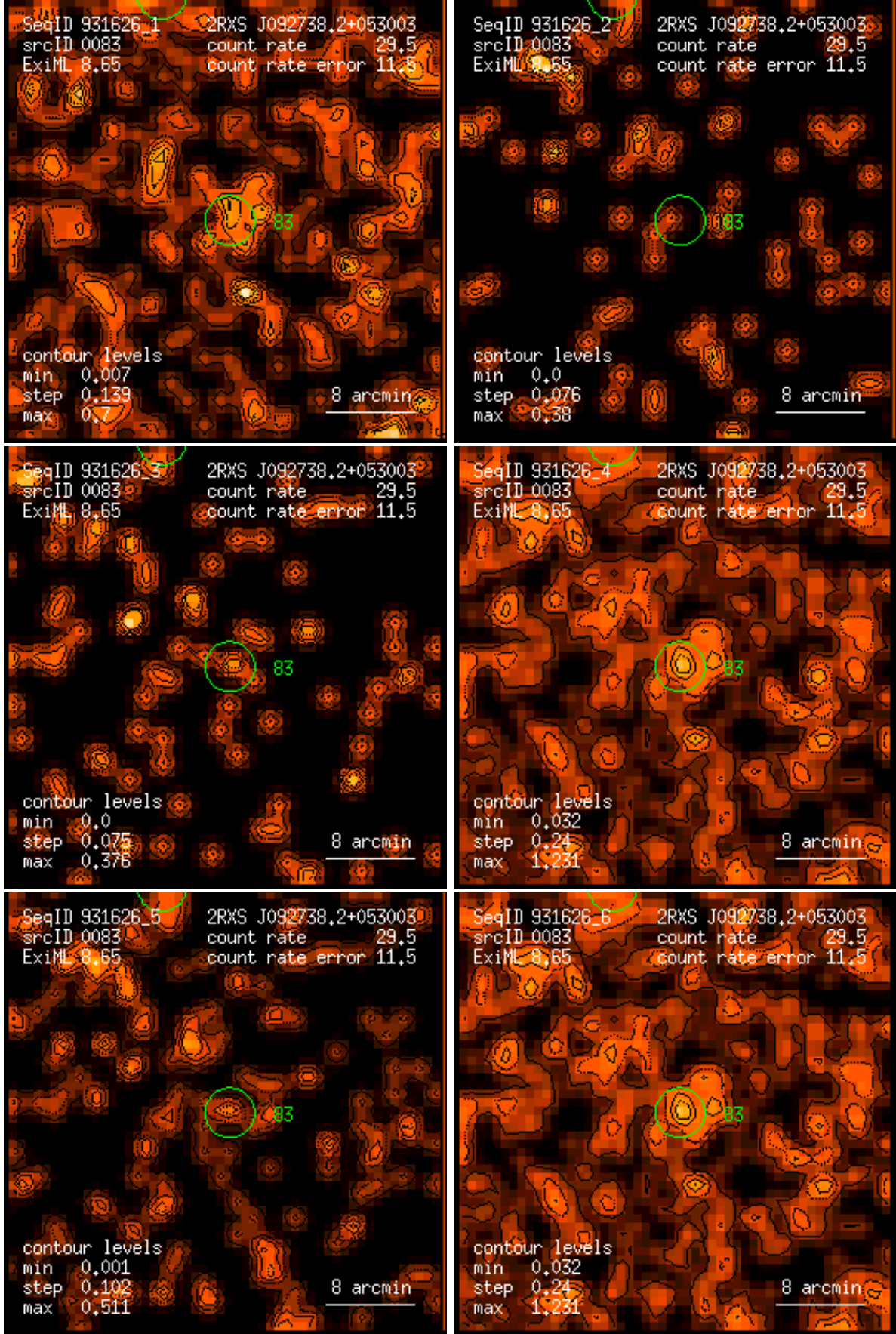
Figure 83: RASS 931626: detection 0083: band rate images, Gaussian filter: (1) PSPC channels 11 – 41, (2) 52 – 90, (3) 91 – 201, (4) 11 – 235, (5) 52 – 201, (6) 11 – 201. Broad band rates in counts/ks. Band rate contour levels in counts/ks/arcmin 2 .
