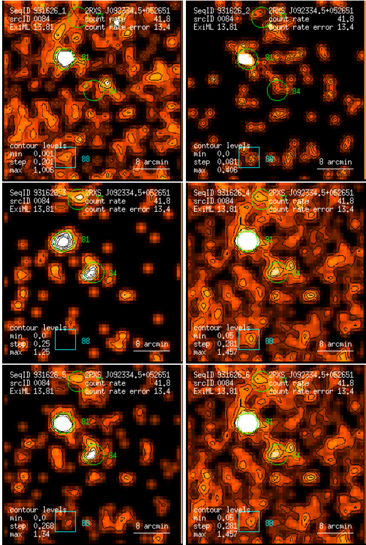
Figure 84: RASS 931626: detection 0084: band rate images, Gaussian filter: (1) PSPC channels 11 – 41, (2) 52 – 90, (3) 91 – 201, (4) 11 – 235, (5) 52 – 201, (6) 11 – 201. Broad band rates in counts/ks. Band rate contour levels in counts/ks/arcmin 2 .
