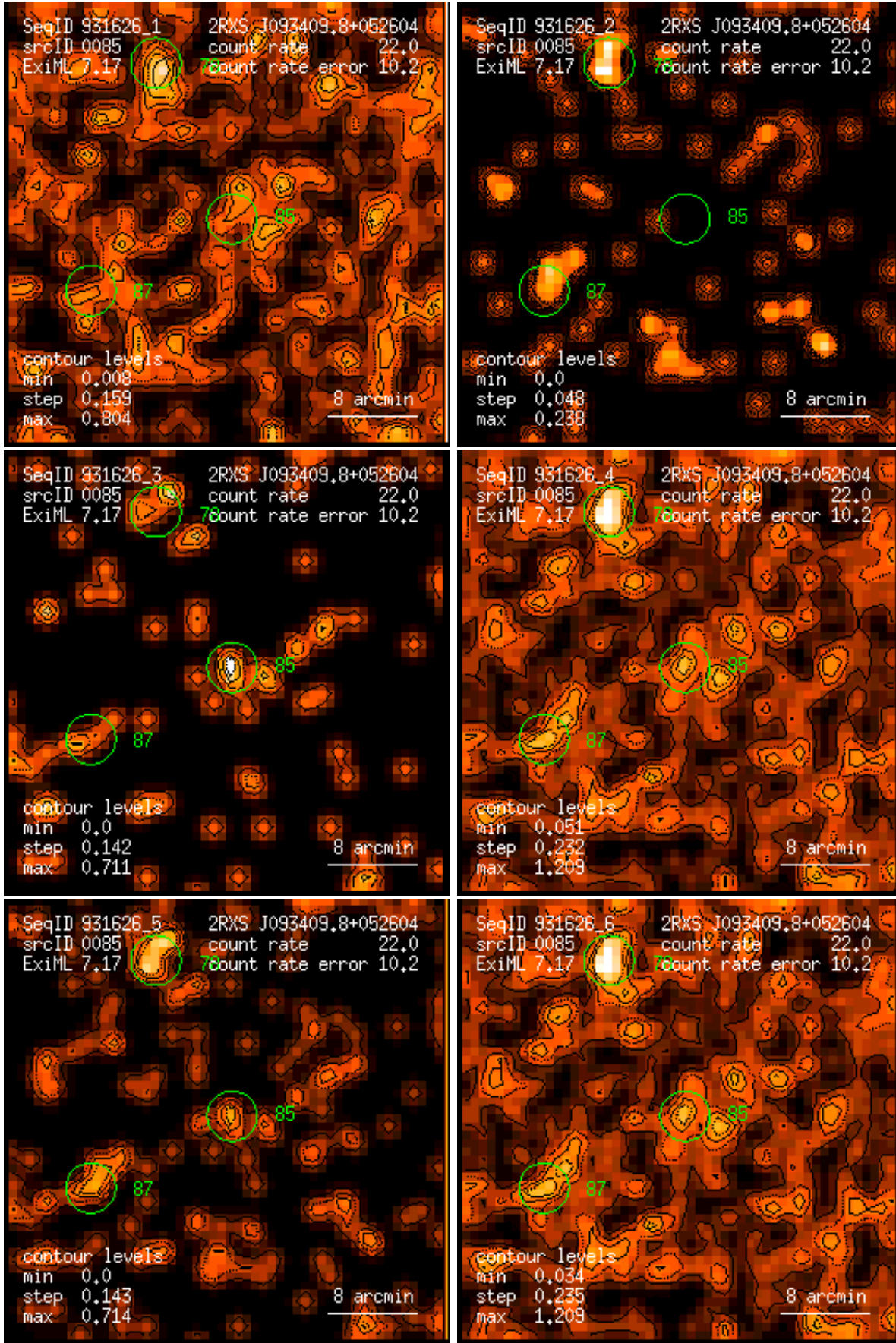
Figure 85: RASS 931626: detection 0085: band rate images, Gaussian filter: (1) PSPC channels 11 – 41, (2) 52 – 90, (3) 91 – 201, (4) 11 – 235, (5) 52 – 201, (6) 11 – 201. Broad band rates in counts/ks. Band rate contour levels in counts/ks/arcmin 2 .
