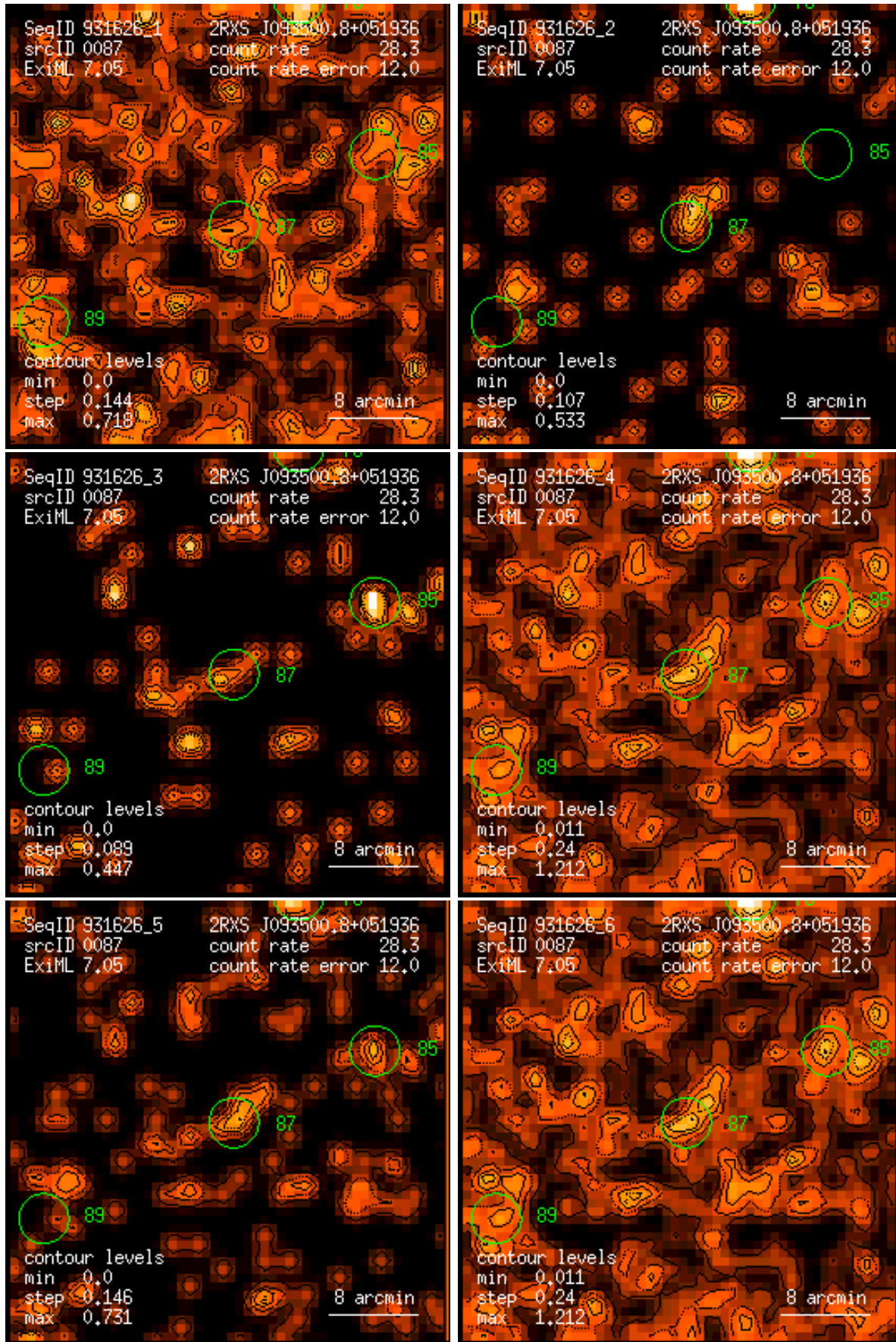
Figure 87: RASS 931626: detection 0087: band rate images, Gaussian filter: (1) PSPC channels 11 – 41, (2) 52 – 90, (3) 91 – 201, (4) 11 – 235, (5) 52 – 201, (6) 11 – 201. Broad band rates in counts/ks. Band rate contour levels in counts/ks/arcmin 2 .
