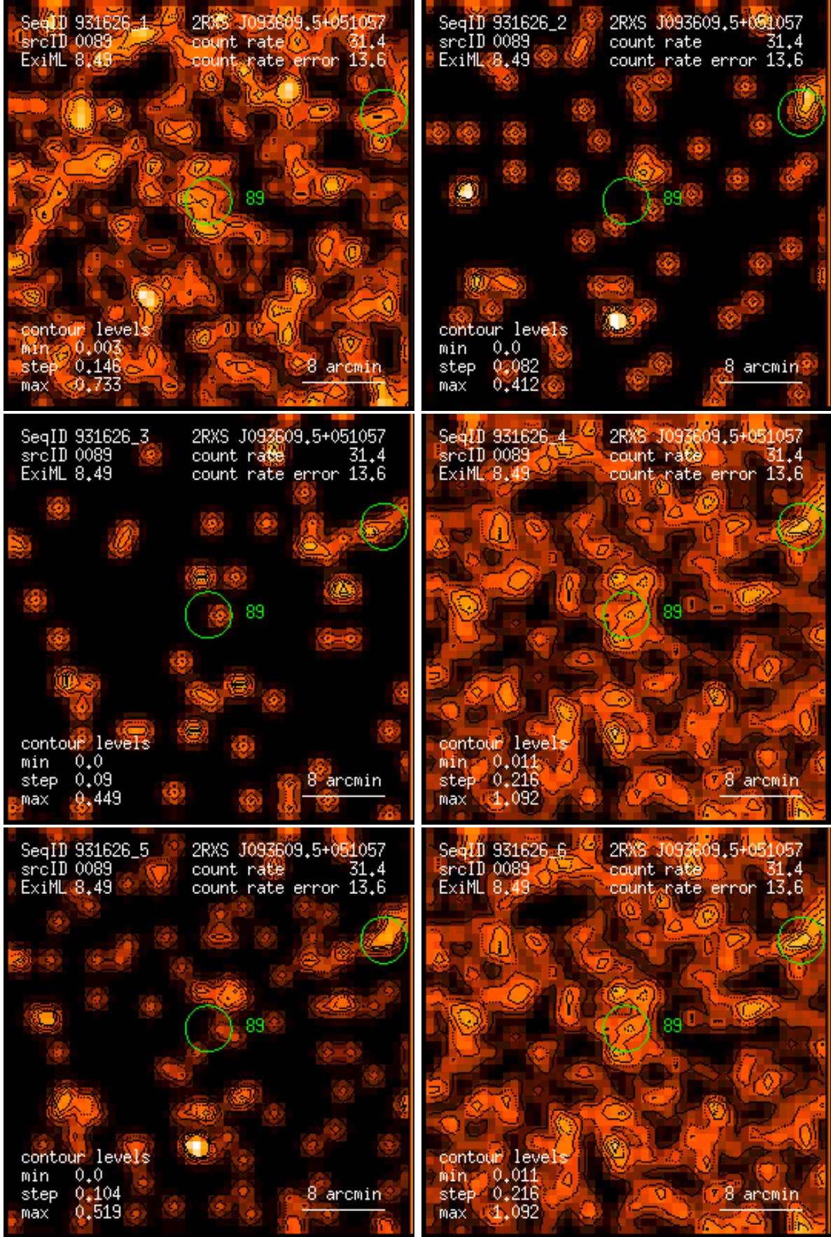
Figure 89: RASS 931626: detection 0089: band rate images, Gaussian filter: (1) PSPC channels 11 – 41, (2) 52 – 90, (3) 91 – 201, (4) 11 – 235, (5) 52 – 201, (6) 11 – 201. Broad band rates in counts/ks. Band rate contour levels in counts/ks/arcmin 2 .
