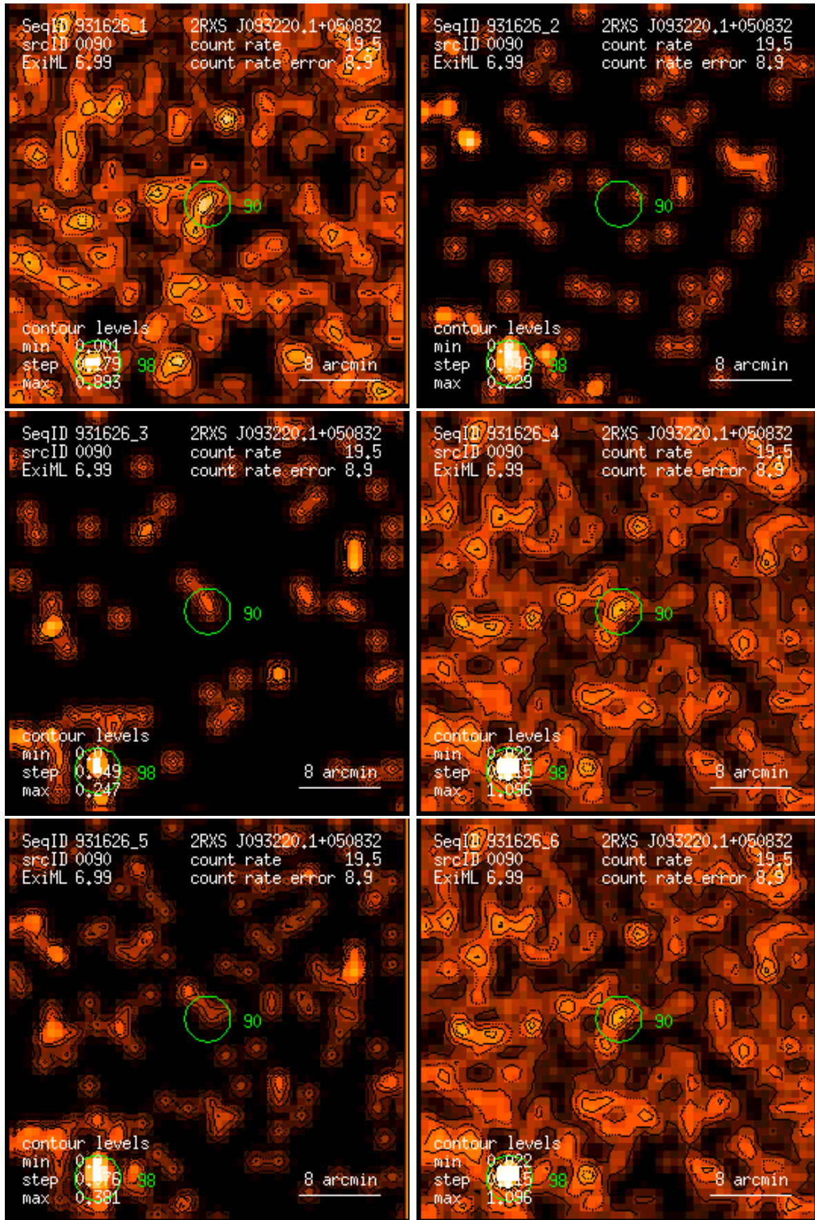
Figure 90: RASS 931626: detection 0090: band rate images, Gaussian filter: (1) PSPC channels 11 – 41, (2) 52 – 90, (3) 91 – 201, (4) 11 – 235, (5) 52 – 201, (6) 11 – 201. Broad band rates in counts/ks. Band rate contour levels in counts/ks/arcmin 2 .
