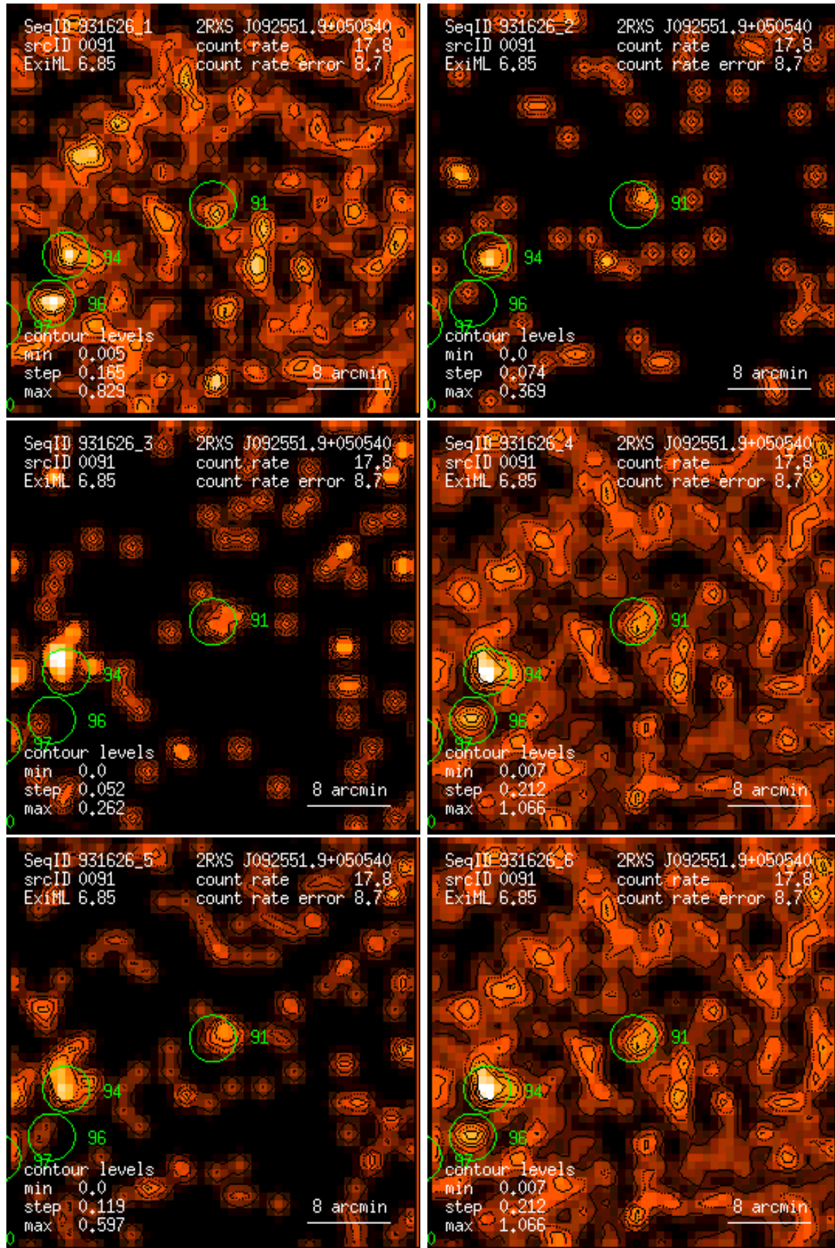
Figure 91: RASS 931626: detection 0091: band rate images, Gaussian filter: (1) PSPC channels 11 – 41, (2) 52 – 90, (3) 91 – 201, (4) 11 – 235, (5) 52 – 201, (6) 11 – 201. Broad band rates in counts/ks. Band rate contour levels in counts/ks/arcmin 2 .
