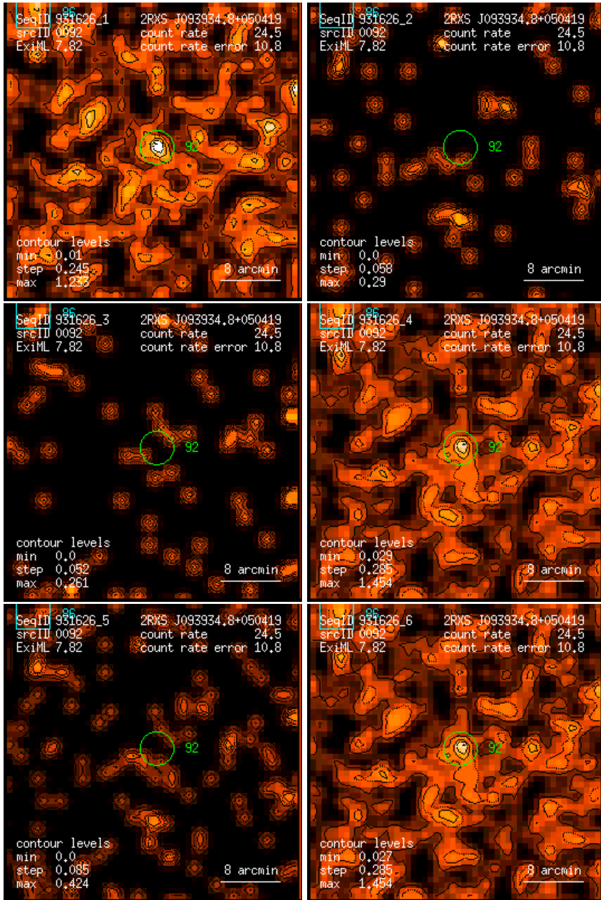
Figure 92: RASS 931626: detection 0092: band rate images, Gaussian filter: (1) PSPC channels 11 – 41, (2) 52 – 90, (3) 91 – 201, (4) 11 – 235, (5) 52 – 201, (6) 11 – 201. Broad band rates in counts/ks. Band rate contour levels in counts/ks/arcmin 2 .
