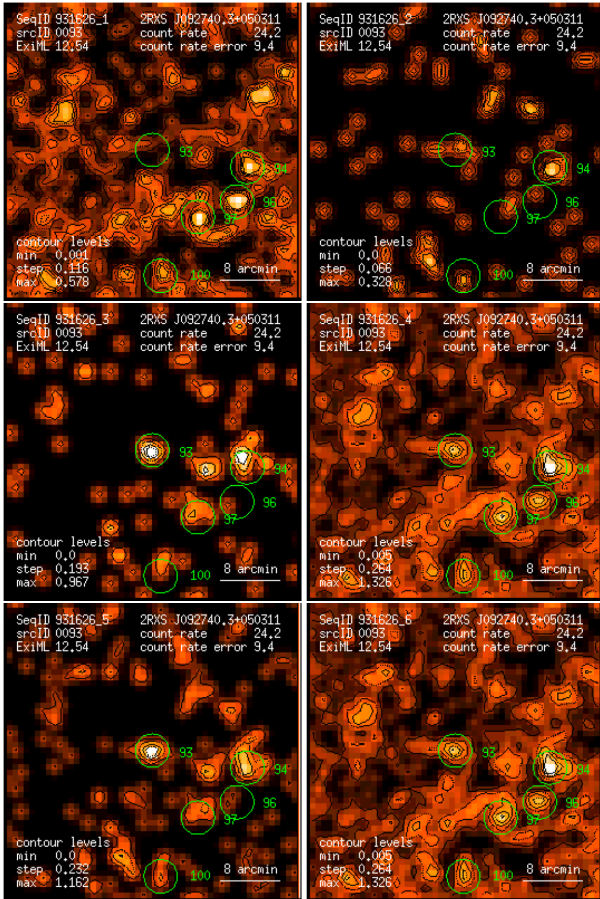
Figure 93: RASS 931626: detection 0093: band rate images, Gaussian filter: (1) PSPC channels 11 – 41, (2) 52 – 90, (3) 91 – 201, (4) 11 – 235, (5) 52 – 201, (6) 11 – 201. Broad band rates in counts/ks. Band rate contour levels in counts/ks/arcmin 2 .
